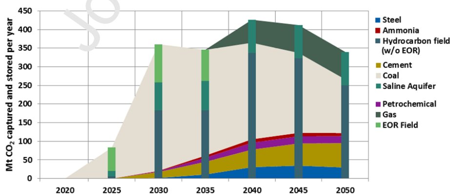
Figure 4: CO 2 storage by sector and storage type in million tCO 2 ( Affordable CCS Scenario )
