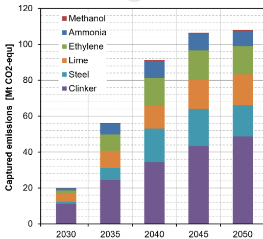
a) EU 28 industrial captured direct CO 2 emissions
