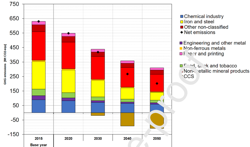
Figure 9: EU 28 industrial direct CO 2 emissions 2015-2050 in the CCS scenarios (Affordable CCS/Costly CCS). Source: FORECAST
