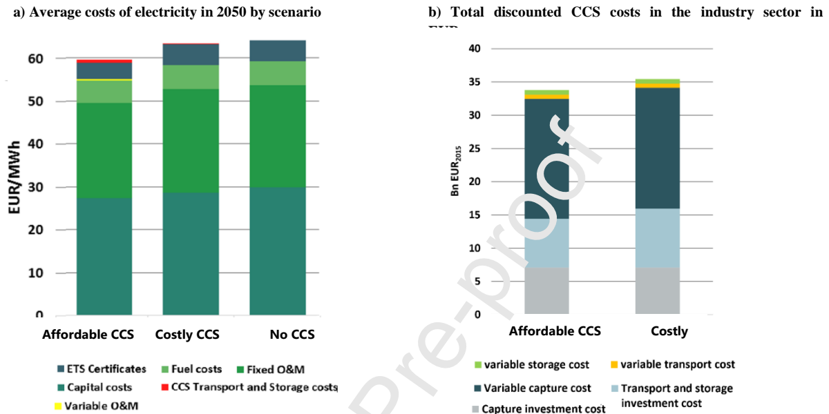
Figure 5: a) Average costs of electricity in 2050 by scenario and b) total discounted CCS costs in the industry sector
