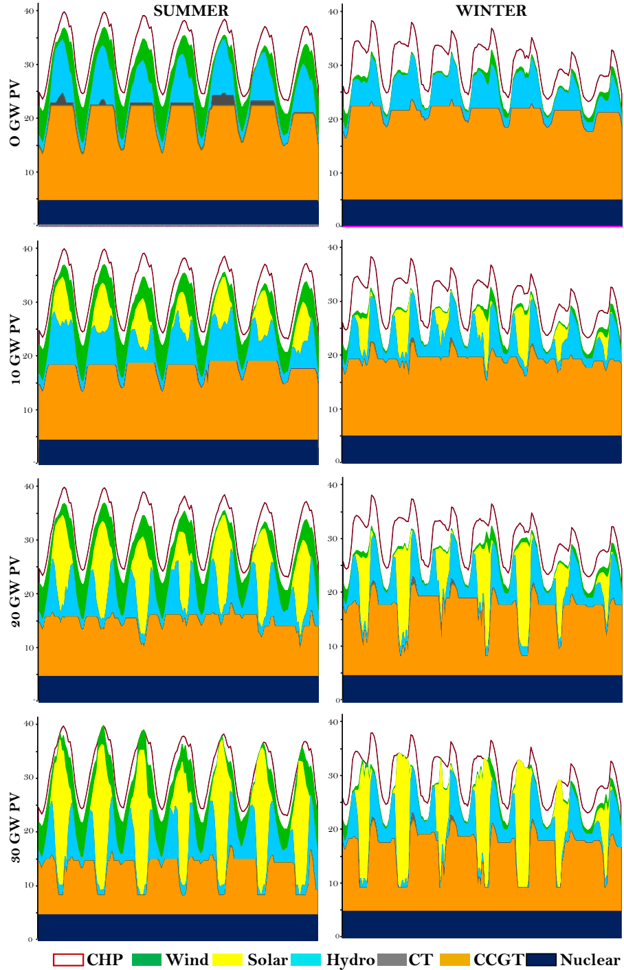
Figure 8. Evolution of the hourly scheduling when the mix can re-adapt (CAISO-like long-term study)
