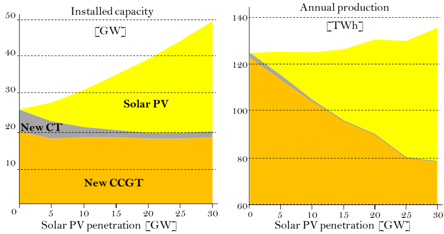
Figure 9- Evolution of the installed capacity and the annual corresponding energy production
