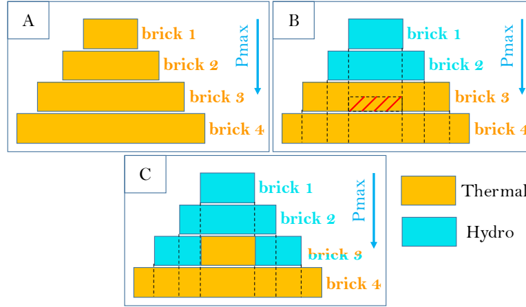
Figure 4. Hydro dispatch when the maximum power output becomes binding
