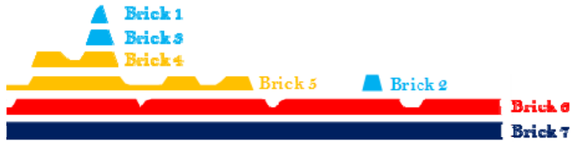
Figure 3. Heuristic hydro dispatch (cost-saving method)
