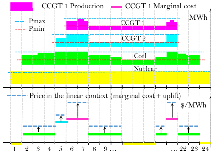
Figure 7. Marginal cost and uplift determination
