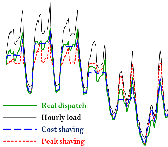
Figure 6. Heuristic approach proposed versus the traditional peak shaving method
