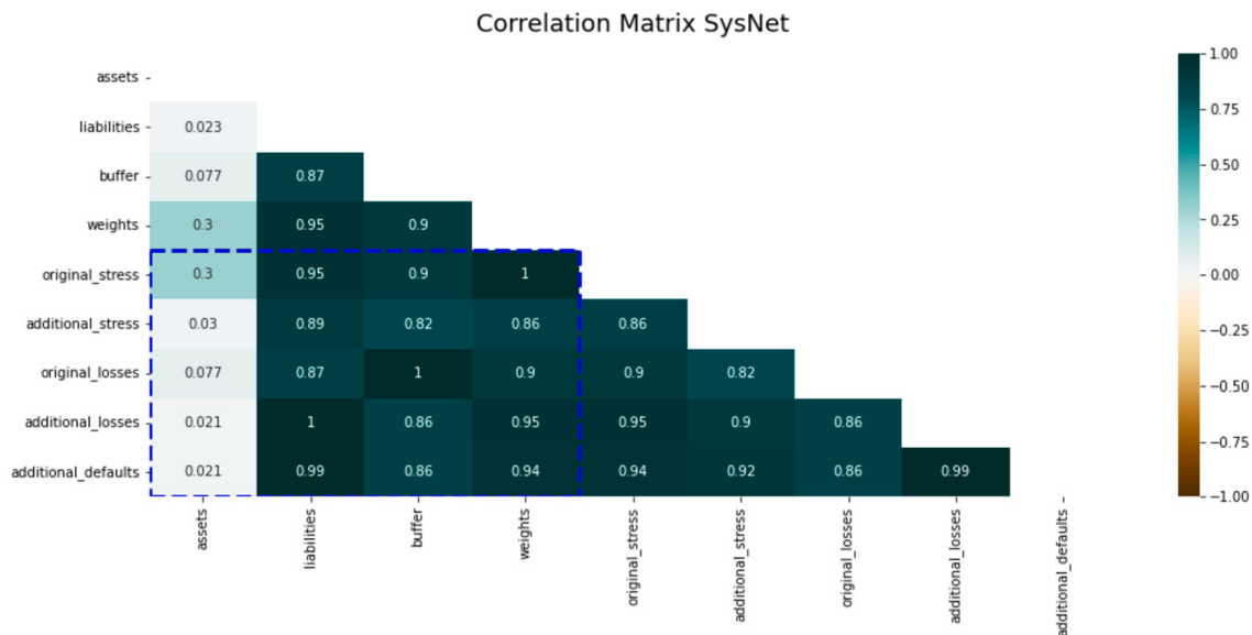
Fig. 3. SymNet correlation of the outputs and inputs of the contagion process.
