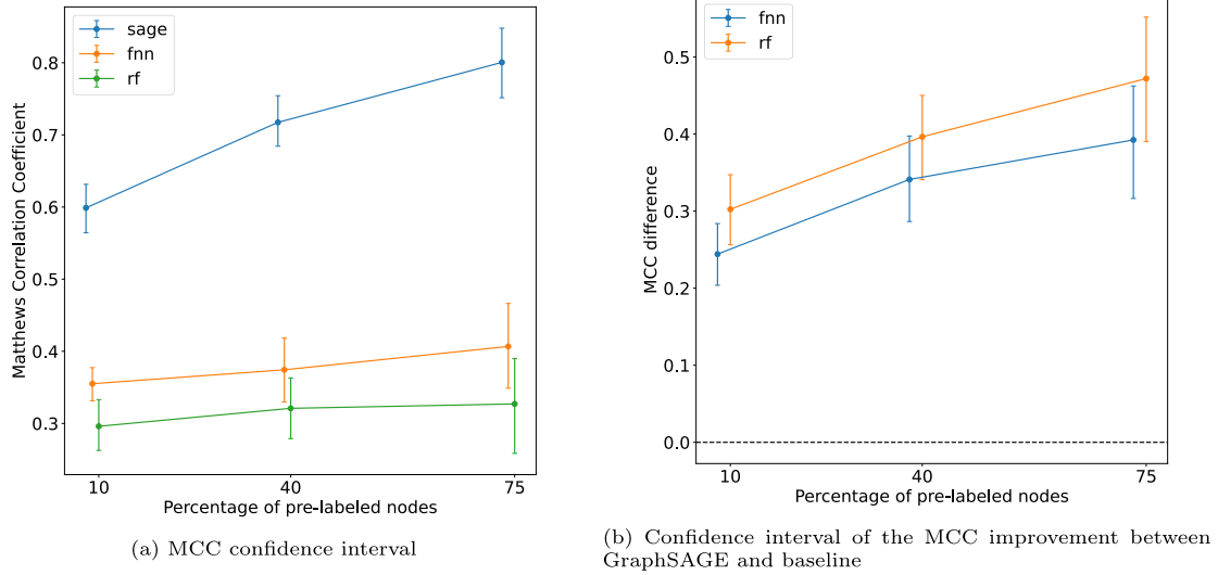
Fig. 10. GraphSAGE achieves statistically significant MCC improvements over the traditional Machine Learning baseline on SymNet.
