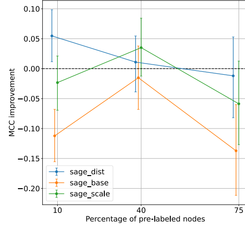
(b) Confidence interval of the MCC improvement between C2R approaches and classification
