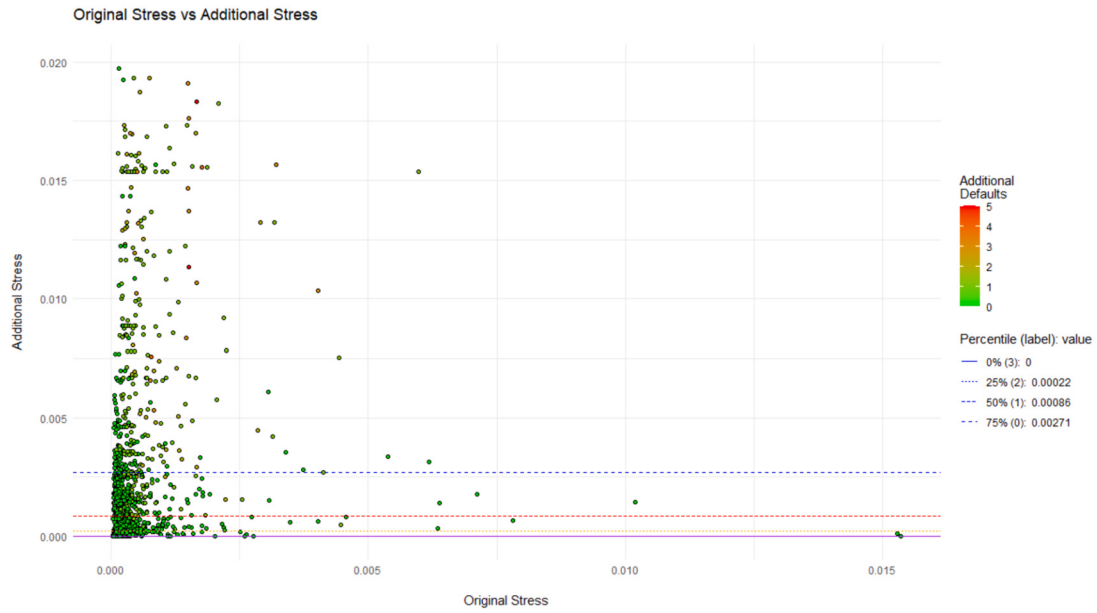
Fig. 4. Symnet original vs additional system stress for smaller nodes.
