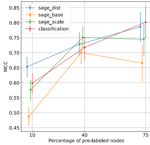
(a) MCC confidence interval
