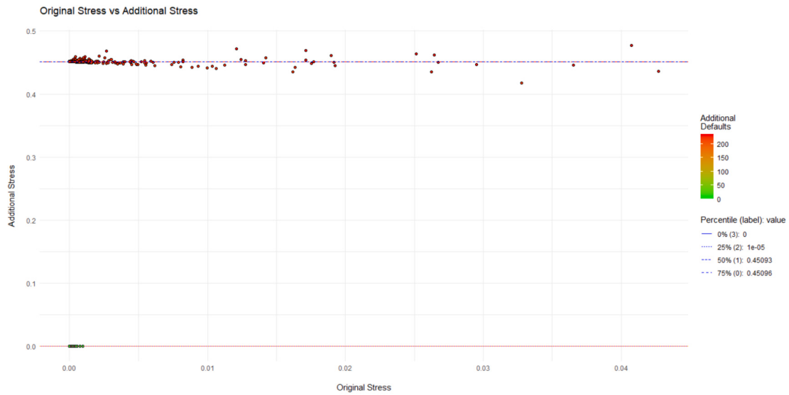
Fig. 7. EurNet original vs additional system stress.
