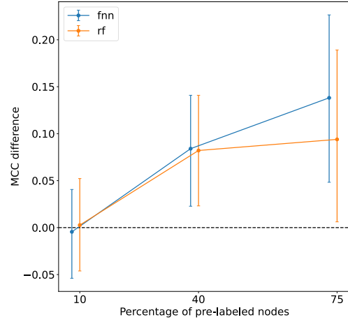
(b) Confidence interval of the MCC improvement between GraphSAGE and baseline
