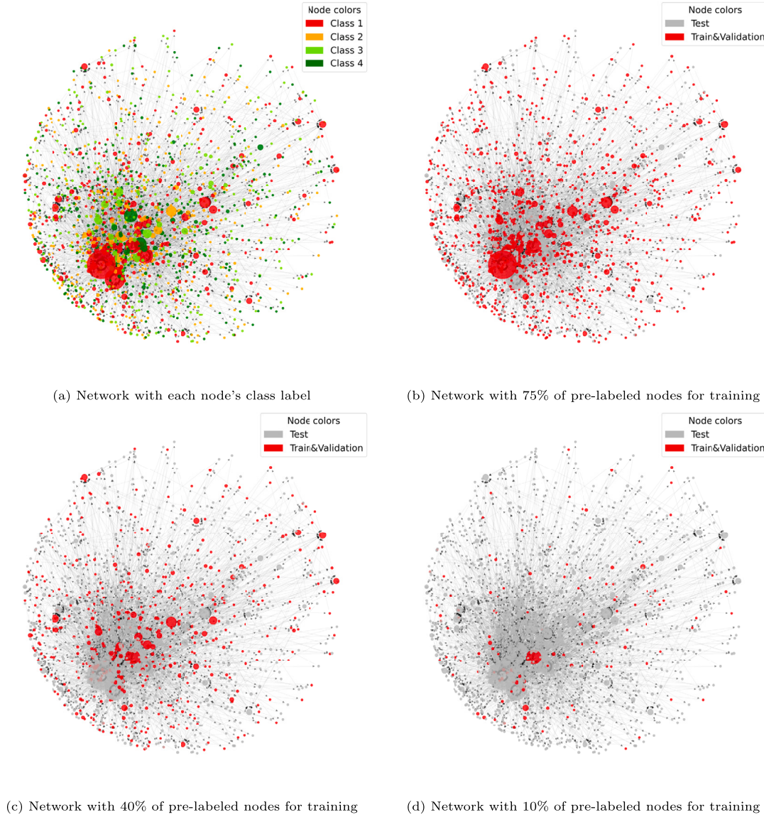
Fig. 8. Representation for the SymNet network. Each circle represents a node, with the size of the circle being proportional to the node's degree.
