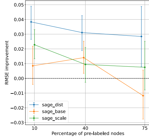
(b) Confidence interval of the RMSE improvement between C2R approaches and classification
