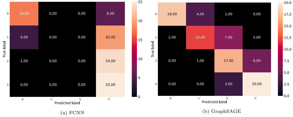
Fig. 11. Normalized confusion matrices for SymNet_10 (percentage of total).
