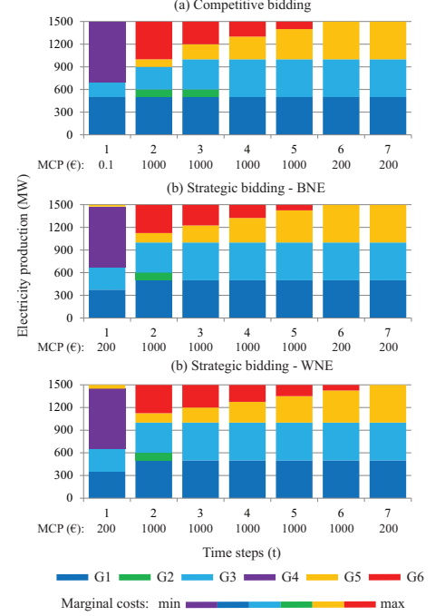
Fig. 2. Short-run economic dispatch and market clearing prices (MCPs) for the cases of (a) competitive and (b) strategic bidding. BNW: best-Nash equilibrium case, WNE: worst-Nash equilibrium case.
