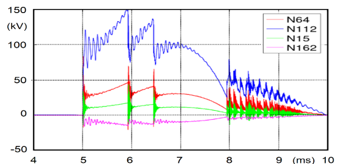
Fig. 8. Transient voltage at various internal nodes of the transformer during VCB closing operation, with a load-side cable length of 224 m.
