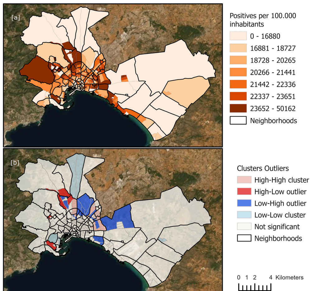
Figure 4. (a) Total geographic distribution of positive cases per 100,000 inhabitants (quartiles), (b) LISA clusters of total cases.
