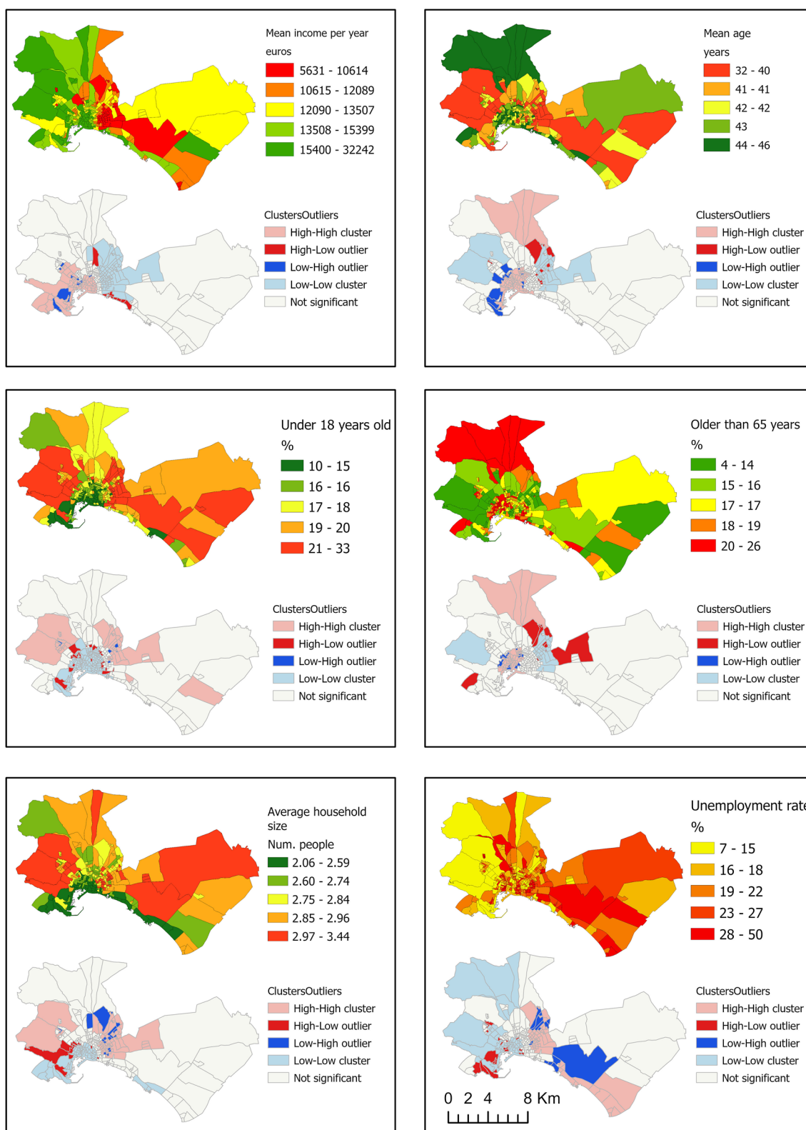
Figure 6. Mapping of socioeconomic variables and its Local Moran's clusters and spatial outliers.
