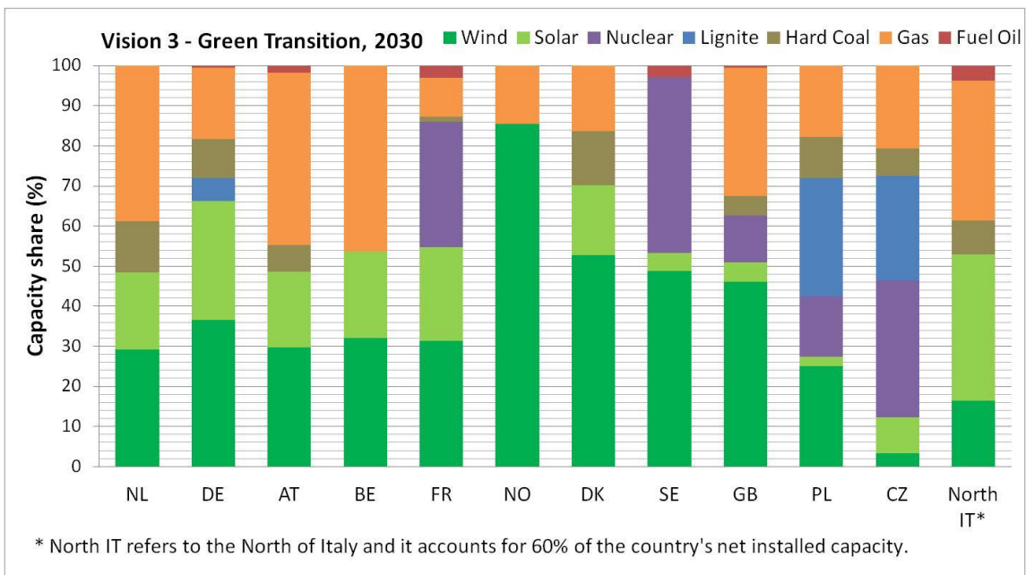
Figure B.2 . Breakdown of generation mix per country in Vision 3 year 2030
