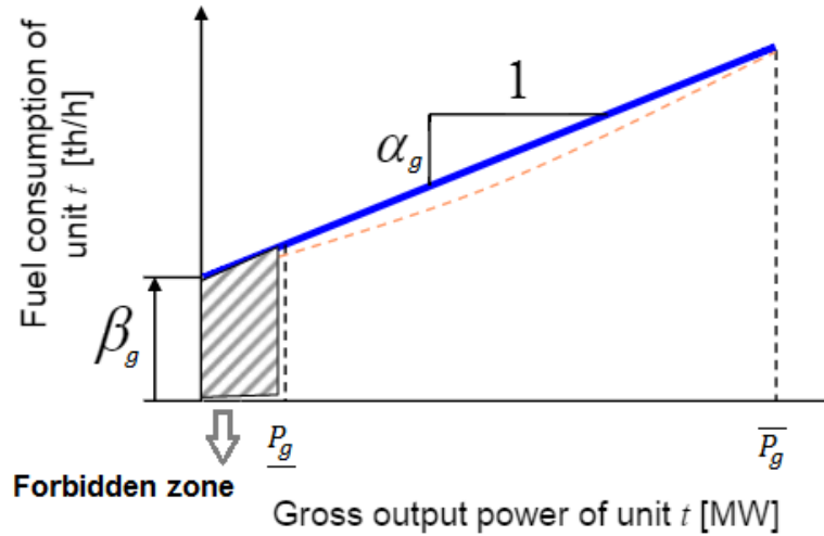
Figure 3.8. Linear approximation of input-output characteristic of generator g . Source: Adapted figure from Comillas University.
