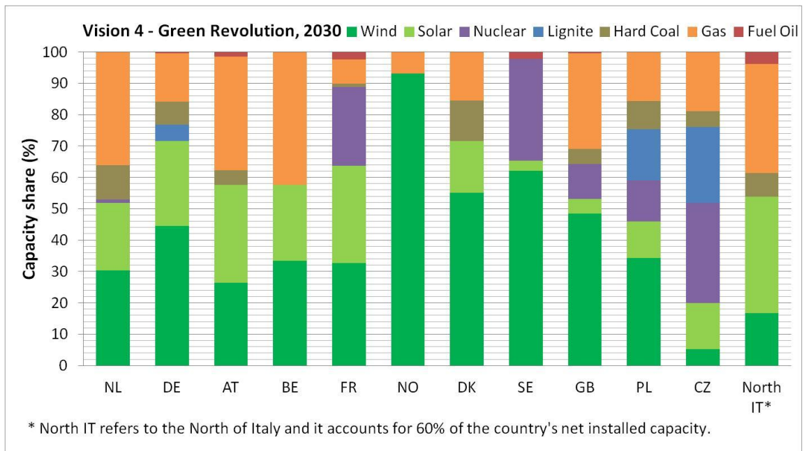
Figure 3.7 . Breakdown of generation mix per country in Vision 4 year 2030. Source: Own source, calculated with the input data in the model.
