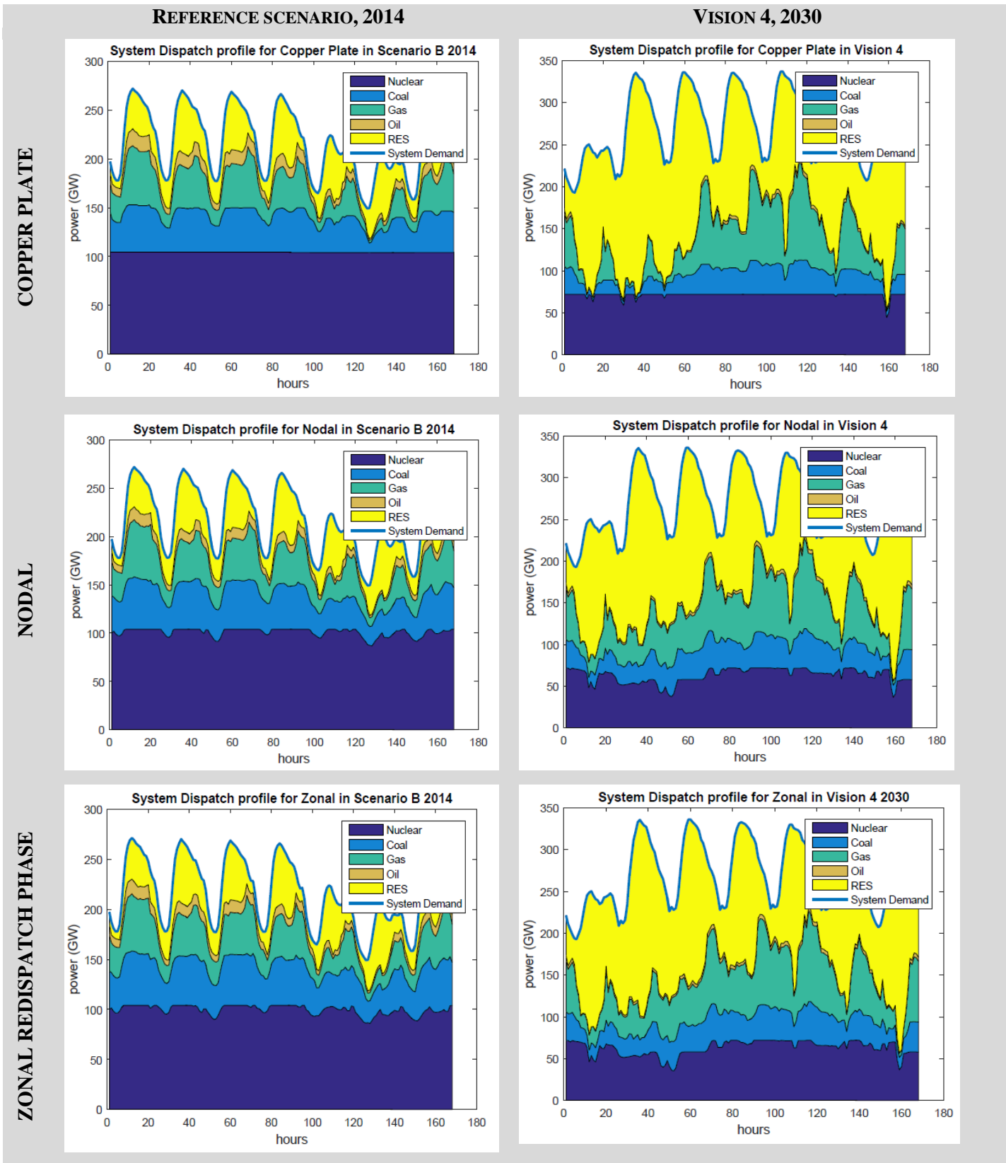
Figure 4.4. Generation dispatch profiles in Reference scenario (2014) and Vision 4 (2030) for the three power market designs
