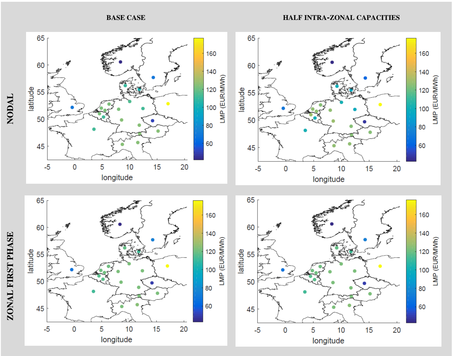
Figure 4.12. Average Locational Marginal Prices in Vision 4 (2030) for the nodal and zonal markets for the base case and half intra-zonal capacities.
