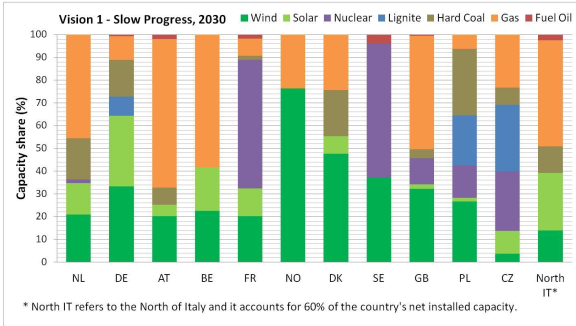
Figure 3.6 . Breakdown of generation mix per country in Vision 1 year 2030. Source: Own source, calculated with the input data in the model.
