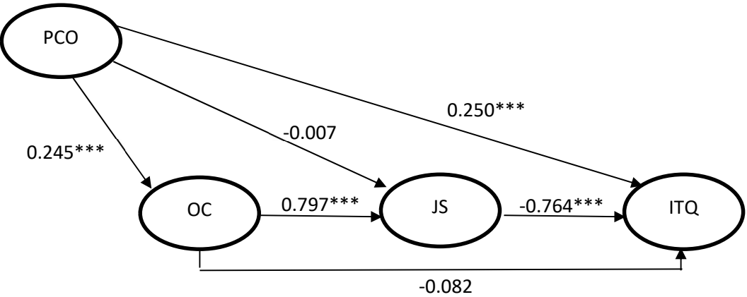
Figure 2: Standardized estimates (direct effects)
