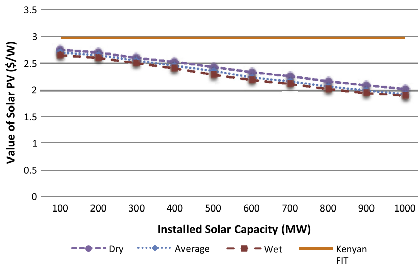
Fig. 4. Economic value of solar PV at different penetration levels in the 2017 National Plan scenario. For all penetration levels and hydrological conditions, the value of solar is below the expected payments from the Kenyan FIT.
