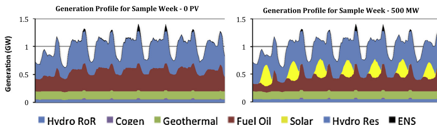
Fig. 1. Changes in system operations as a result of 500 MW solar penetration over a sample 1 week period in the 2012 scenario. Generation from diesel is displaced by solar generation during the day and by shifted hydropower generation during the evenings and night.
