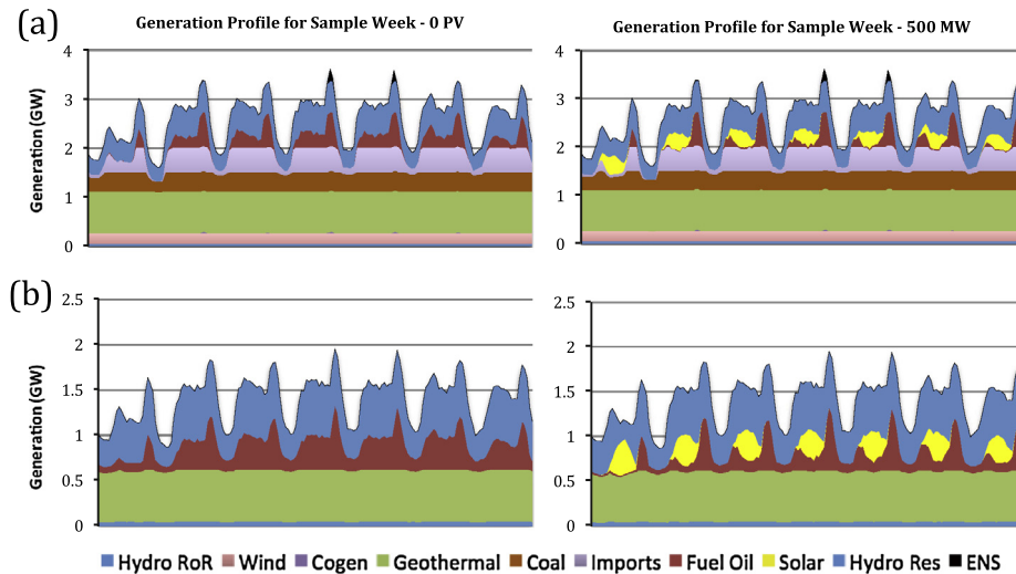
Fig. 3. Changes in system operations as a result of 500 MW solar penetration over a sample 1 week period in the 2017 (a) National Plan, (b) Slow Growth scenarios.
