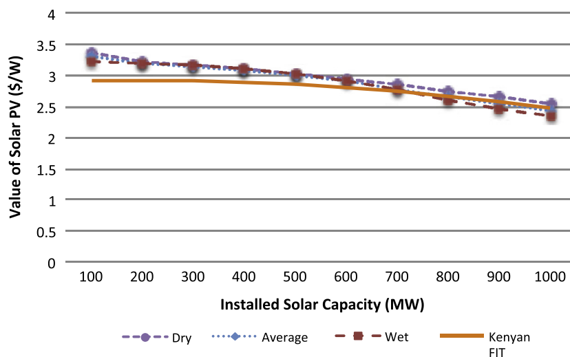
Fig. 5. Value of solar PV in the 2017 Slow Growth simulated year. The value of solar is above the expected payments from the Kenyan FIT up to 700 MW. At higher penetration levels, both the value of solar and expected FIT payments decline because solar is curtailed.
