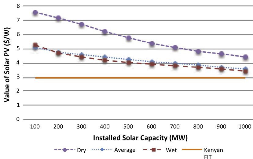
Fig. 2. Economic value of solar PV based different penetration levels in the 2012 simulated year. The value for dry years is higher the value for wet and average hydrological years for all penetration levels. The values for all penetration levels and hydrological conditions are higher than the expected payments from the Kenyan FIT.
