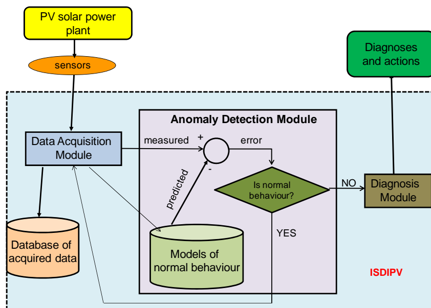
Figure 1. ISDIPV architecture.
