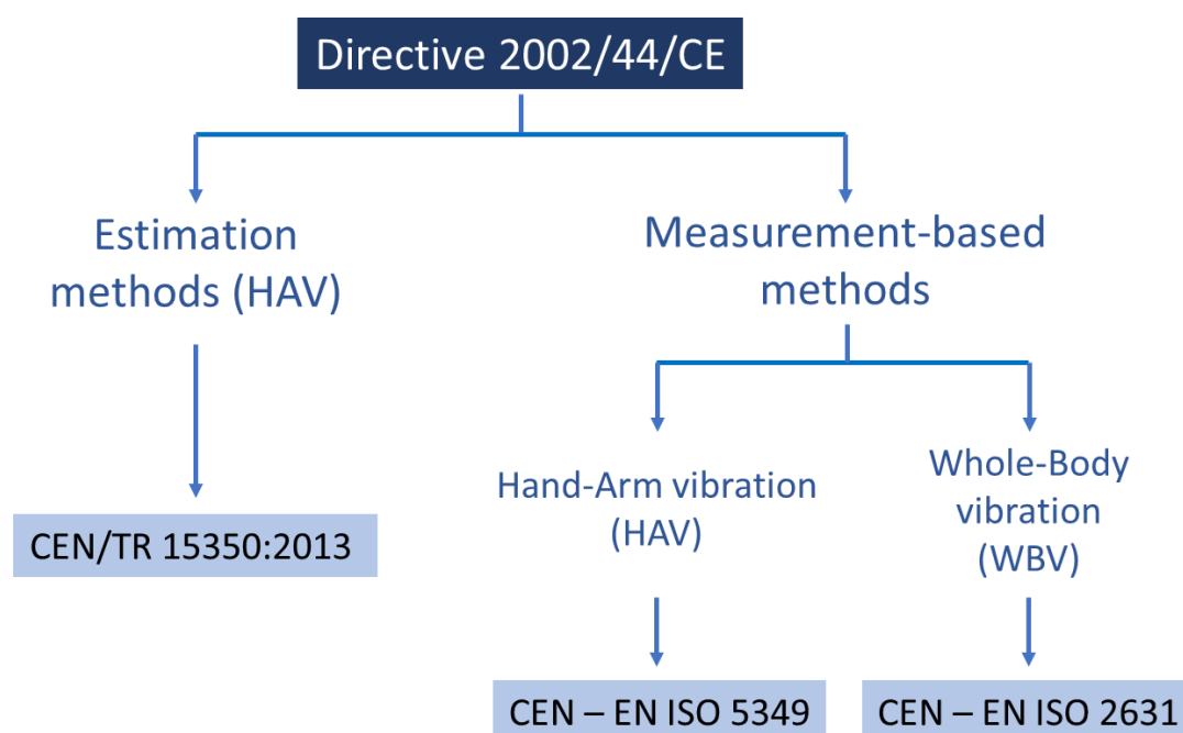
Figure 2. Schematic view of the applicable technical regulations for hand-arm transmitted vibration (HAV) and whole-body vibration (WBV).
