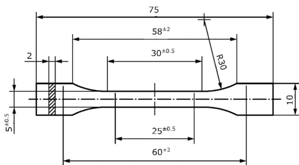
Figure 1. Geometry and size of the specimens according to ISO 527-2 (2012). Distances are given in millimeters (mm).
