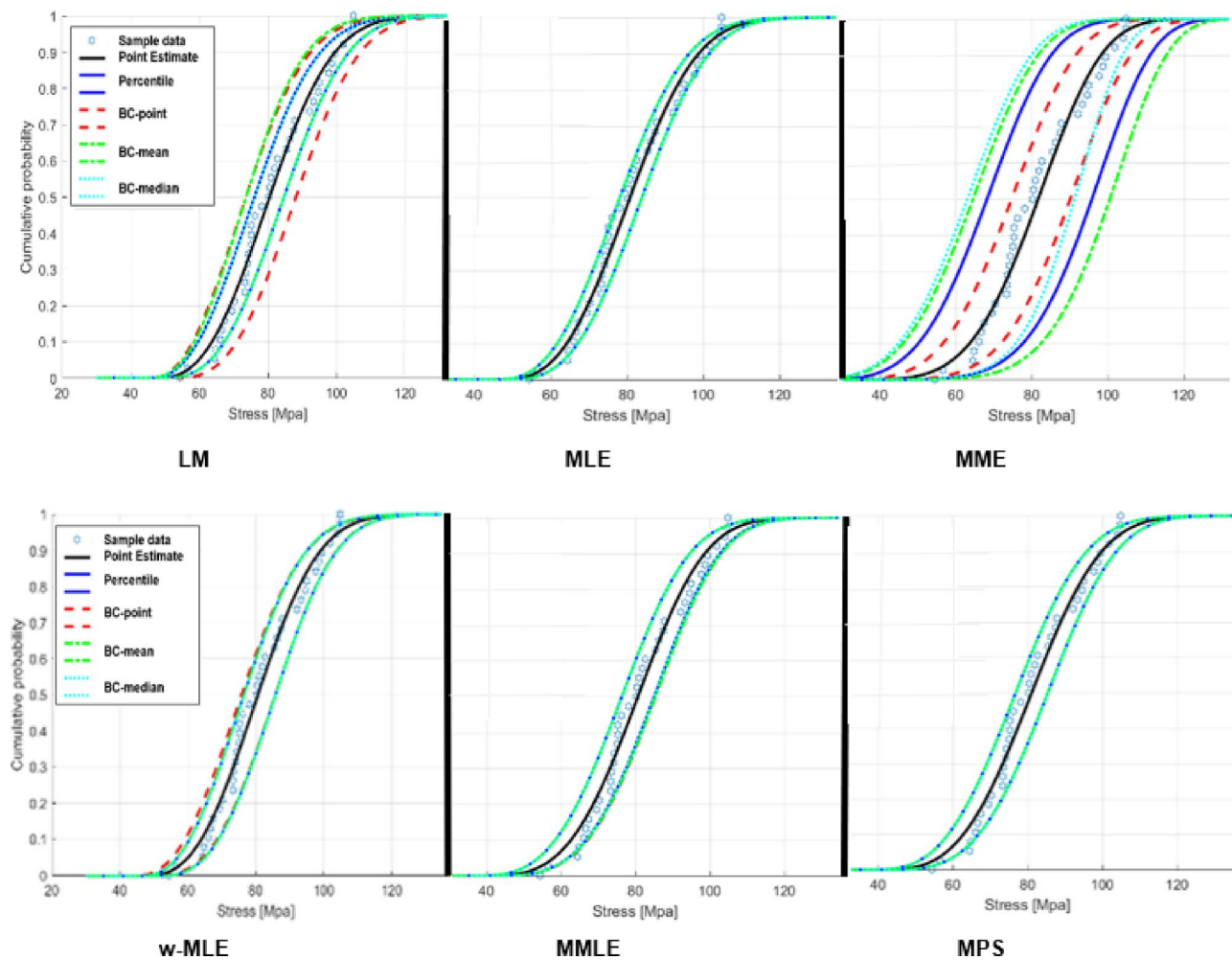
Figure 3. Reliability curves of the Weibull distribution according to bootstrap CIs from the percentile and bias-corrected approaches. Number of subsamples = 100.
