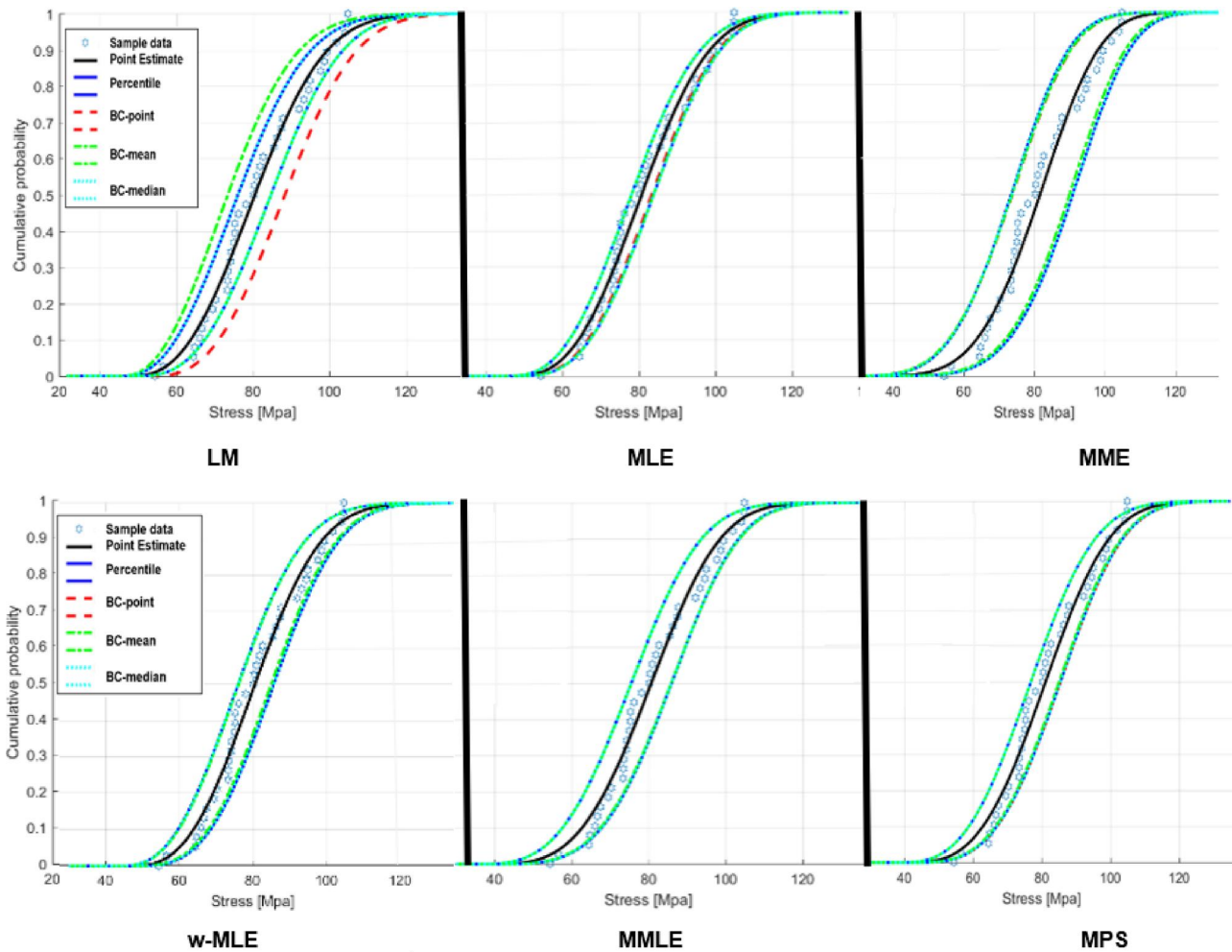
Figure 2. Reliability curves of the Weibull distribution according to bootstrap CIs derived from the percentile and bias-corrected methods. Number of subsamples = 39.
