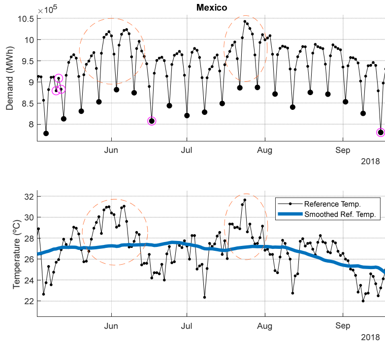
200 Fig. 4. Example of variations in the daily demand of Mexico due to temperature. Top: real demand, the magenta circles mark holidays. Bottom: Reference temperature (black) and smoothed reference temperature (blue).
