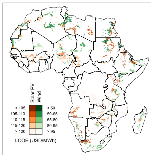
a MSRs by LCOE
