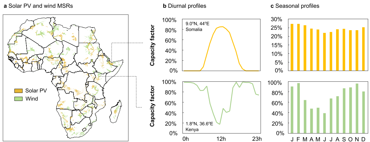
Fig. 3 Spatial distribution of solar PV and wind MSRs across Africa. (a) A map of the African continent showing all solar PV and wind MSRs screened by LCOE up to a maximum coverage of 5% of a country's area. (b,c) Example temporal profiles (diurnal and seasonal) for the two example locations indicated in (a) . The diurnal example in (b) covers the 12th day of March.
