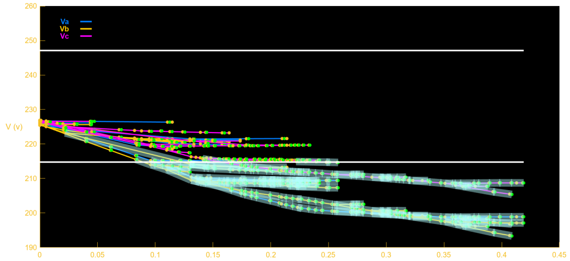
(c) N5 Base Case Voltage Profile
