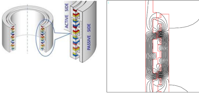
Fig. 5. (a) The concept of a 3 Phase Linear Cylindrical Switched Reluctance Machine (CSRSM). (b) Magnetic flux-lines calculated with FEM.
