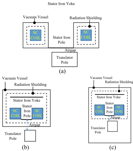
Fig. 3. (a) Only SC Coils working at cold. (b) Full Stator working at cold. (c) Full Stator & Translator working at cold.
