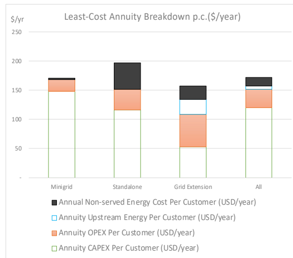
Figure 8. CAPEX, OPEX, upstream energy, and CNSE breakdown of the annual cost of supply (annuity in USD/year) per electrification mode.
