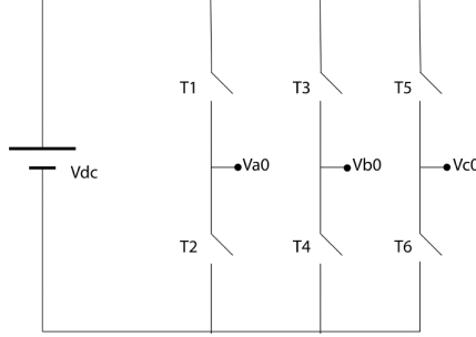
Figure 1: Scheme of a three-phase inverter. V_{dc} is the continuous input voltage, V_{a0} , V_{b0} and V_{c0} are the alternating output voltages.
