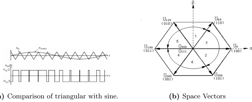
Figure 2: Obtaining PWM signals.
