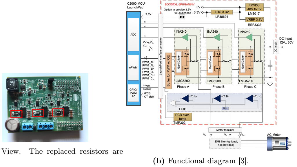
Figure 6: BOOSTXL-3PhGaNInv. .
