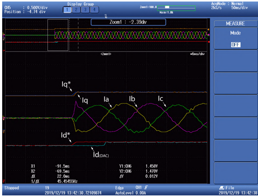
Figure 8: Three-phase currents through the inductances. Axis d and axis q currents. Application of references simultaneously. Step changes in I_d and I_q set points are applied simultaneously. All signals are identified in the figure.
