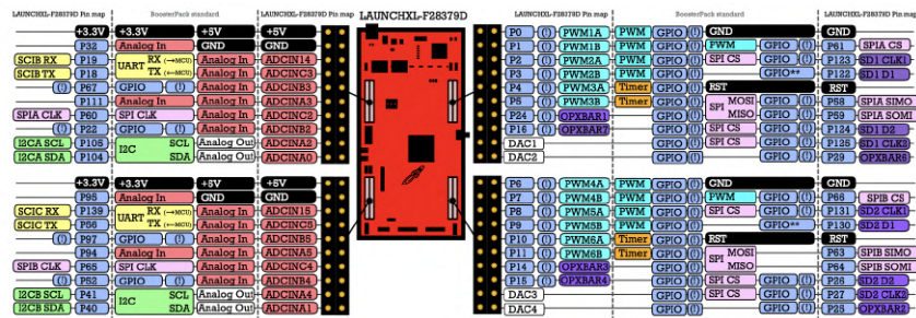
Figura 6.8: Tarjeta LAUNCHXL - F28379D Pinout [45].
