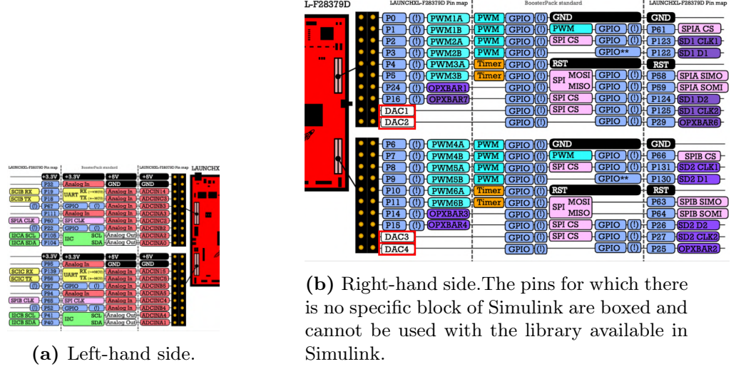
Figure 5: Pinout detail view of the LAUNCHXL card - F28379D. [2].
