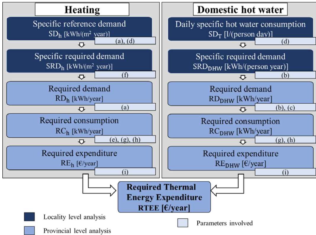
Fig. 1. Flowchart of the Required Thermal Energy Expenditure methodology (the parameters involved in the calculation are listed in the text)
