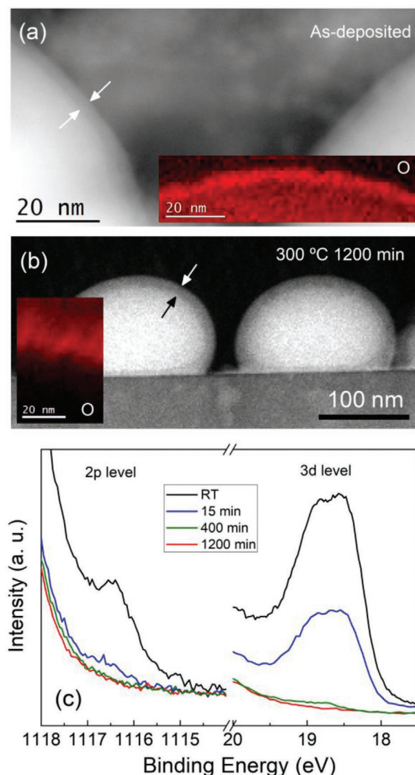
Figure 4. Z-contrast STEM images of the a) as-deposited and the annealed sample at b) 300 °C for 1200 min where the liquid Ga core and the \text{Ga}_x\text{O}_y shell (arrows) can be identified. Insets display the oxygen (red-colored) EELS. c) XPS spectra of Ga 2p (left) and Ga 3d (right) levels for the samples oxidized at 300 °C during different times, including the as-deposited sample. Note, that the Ga 2p peak is superimposed on the tail of the larger Ga-O peak.
