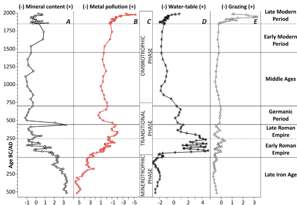
Fig. 3. Compilation of the main results obtained in previous studies on La Molina mire for the last c. 2500 years. A) Mineral content of the peat, a proxy for catchment soils erosion (PC1 factor scores of the geochemical data; Martínez Cortizas et al., 2013); B) atmospheric metal pollution index, proxy for mining and metallurgy (PC2 factor scores of the geochemical data, note that the X axis has been inverted, Martínez Cortizas et al., 2013); C) local wetland phases (López-Merino et al., 2011); D) water-table level index (sum of PC1, PC7, PC4, PC6, PC3 and PC8 factor scores of the hydro-hygrophytes and NPP data, as they are related to fluctuations in the water-table levels, data from López-Merino et al., 2011); E) grazing index (PC2 factor scores of the hydro-hygrophytes and NPP data, related to coprophilous fungi, López-Merino et al., 2011).
