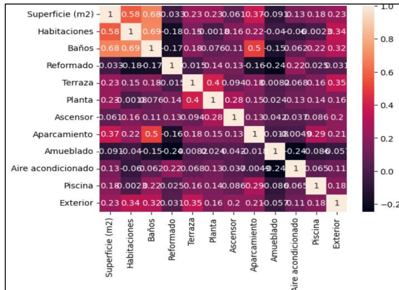
Illustration I: Correlation matrix
