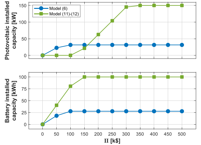
Fig. 7. The PV-BES installed capacity for various budgets using the models (6) and (11)–(12).
