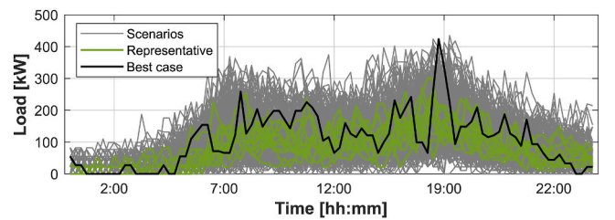
Fig. 2. Illustrative example about the importance of considering the best-case scenario. As seen, the representative profiles do not capture some important features of the best-case profile.
