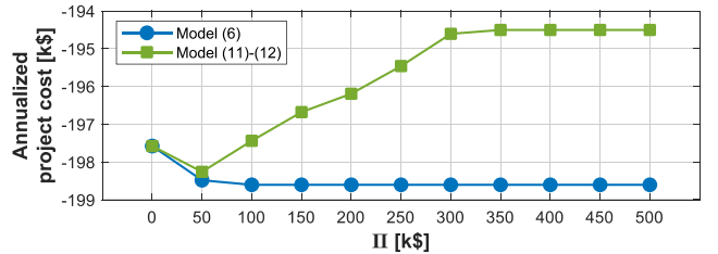
Fig. 8. Total annualized project cost for various budgets.
