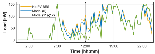
Fig. 12. Power imported from the grid with various PV-BES layouts. In the case of models (6) and (11)–(12), results correspond with \Pi = 400 k$.
