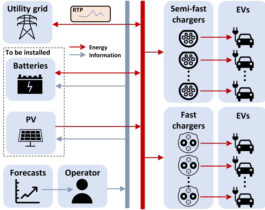
Fig. 1. Schematic representation of the studied multi-mode charging station.
