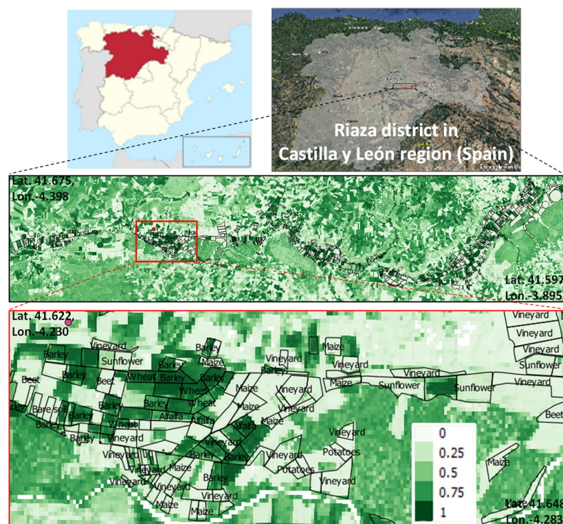
Figure 1. Top panel: Castilla y León region in Spain and the Riaza irrigation district location. Middle panel: zoomed-in view of the black rectangle with parcel borders overlayed on the S-2 NDVI on 30 April 2019. Red point indicates the VA07 Inforiego meteorological station. Bottom panel: zoomed-in view of the red rectangle with crop type information. Geographic coordinates of the corners are reported.
