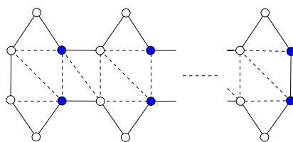
Fig. 2. A maximal outerplanar graph G such that \gamma_{t2}(G) \geq \lfloor \frac{n}{3} \rfloor .
