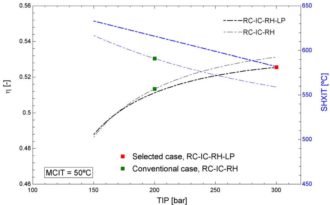
Fig. 11. Performance comparison between selected layouts of the novel cycle and the conventional layouts when dry cooling is used.
