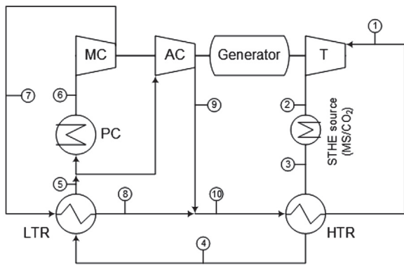
(b) Novel recompression cycle (RC-LP)
