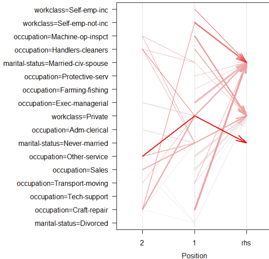
Parallel coordinates plot for 30 rules
