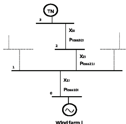
Fig. 1. Diagram of the distribution network
