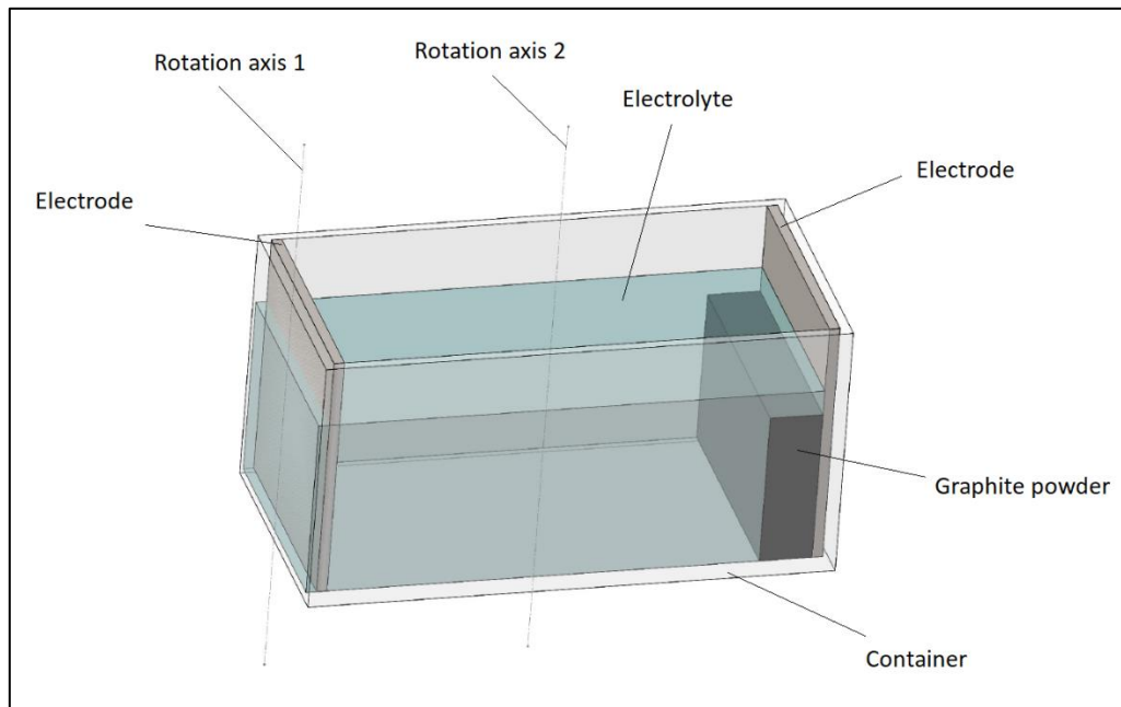
Figure 15: Rectangular centrifugation-assisted design
