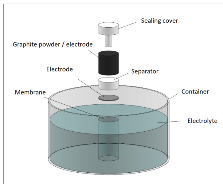
Figure 24: Pressurized design
