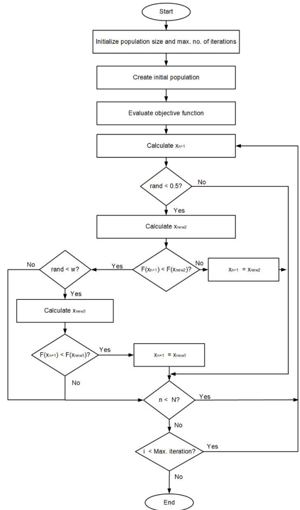
FIGURE 4. Flow chart of the RUN optimization algorithm.
