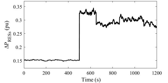
FIGURE 15. RESs power variation for scenario 3.
