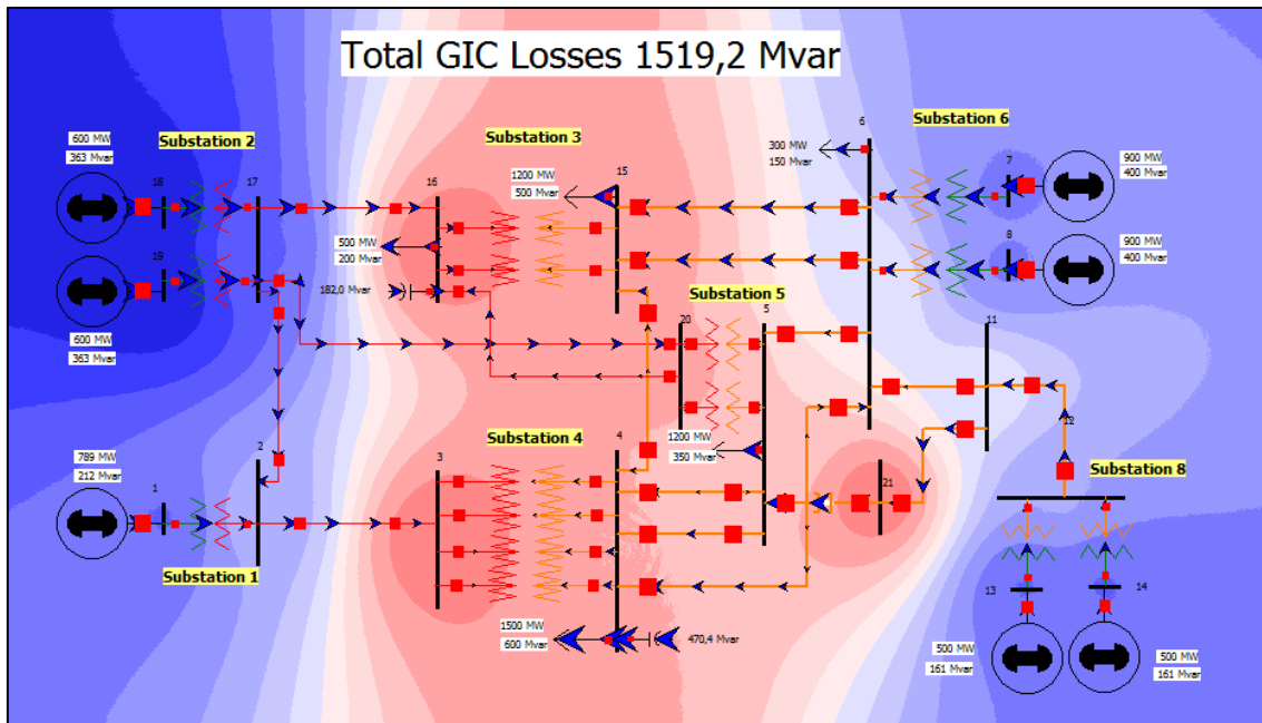
Figure 29 21 Bus system under 7 V/km
