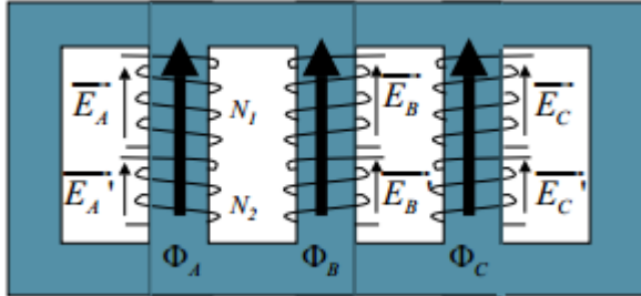
Figure 8 Five legged transformer [10]
