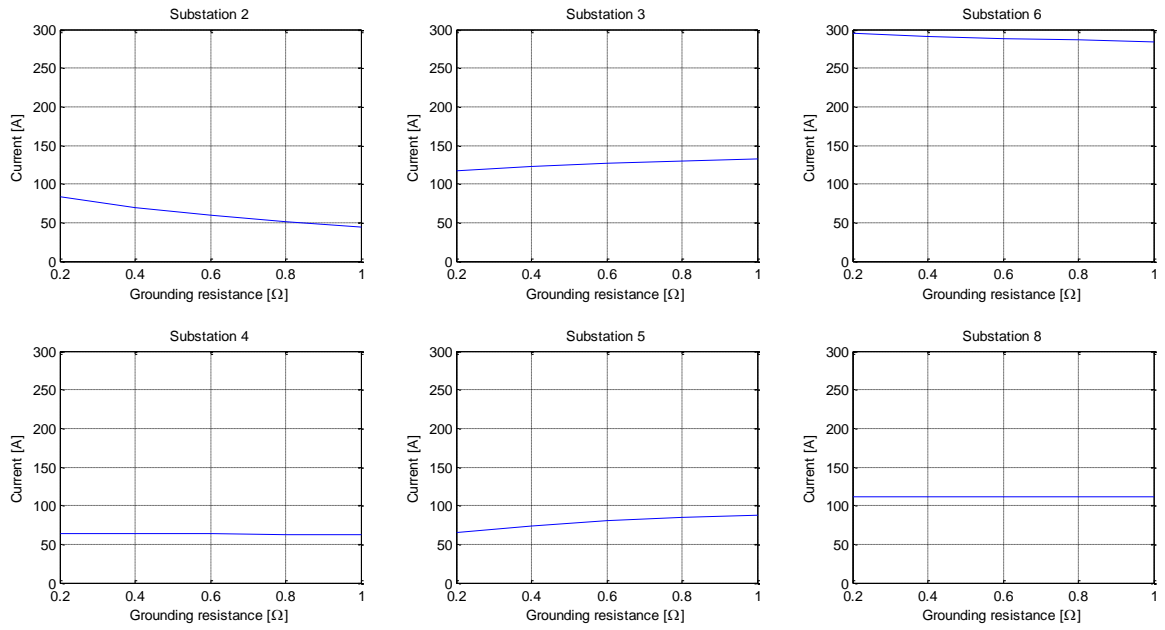
Figure 35 Induced current in different busses when modifying resistance in substation 2, equal scales.
