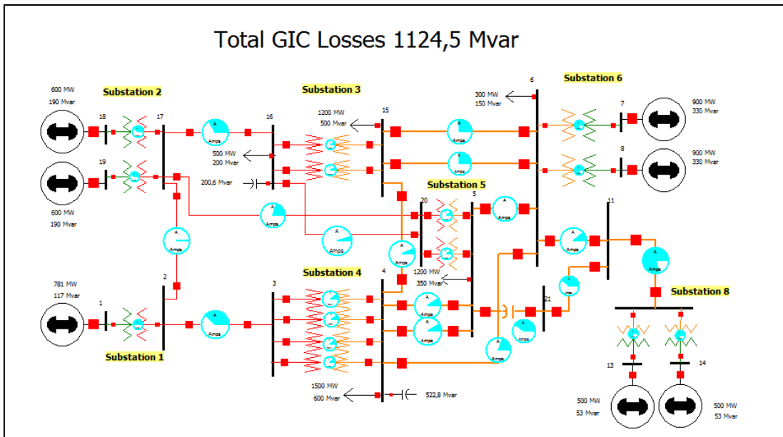
Figure 43 21 Bus system, all transformers and lines.
