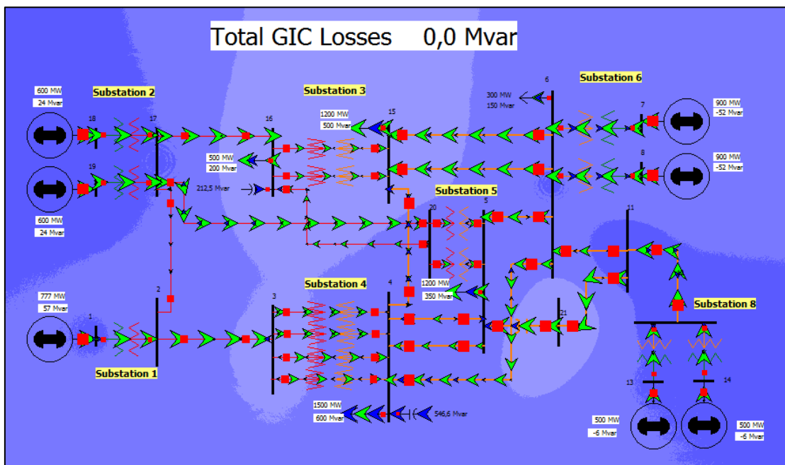
Figure 3 21 bus test system with no GIC.
