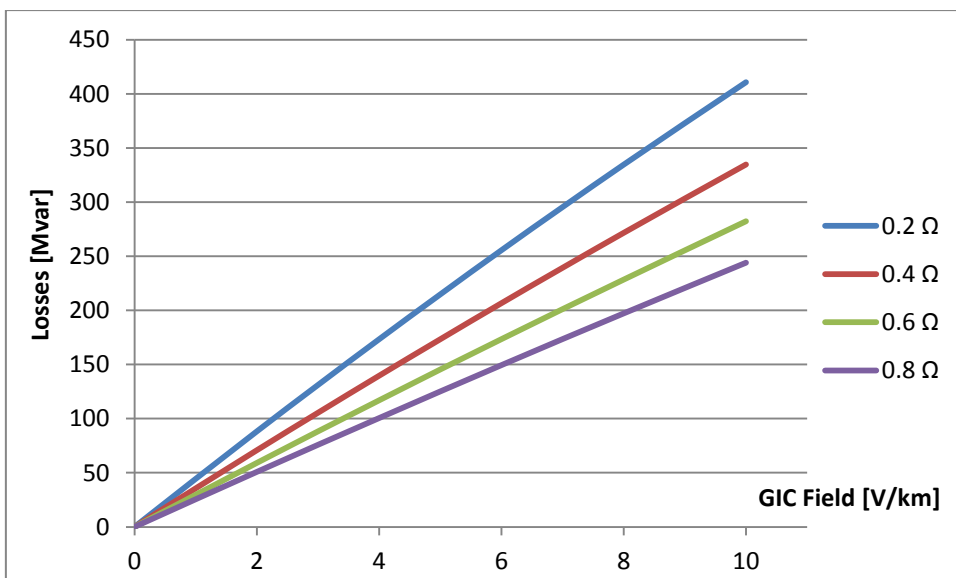
Figure 24 Reactive losses for different grounding resistance in a three-legged shell transformer.
