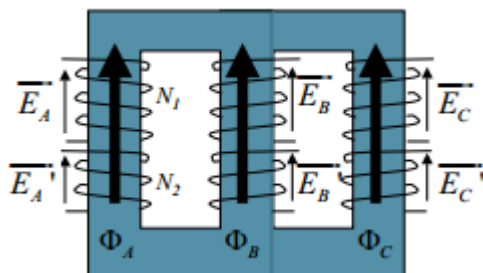
Figure 7 Three legged transformer [10]
