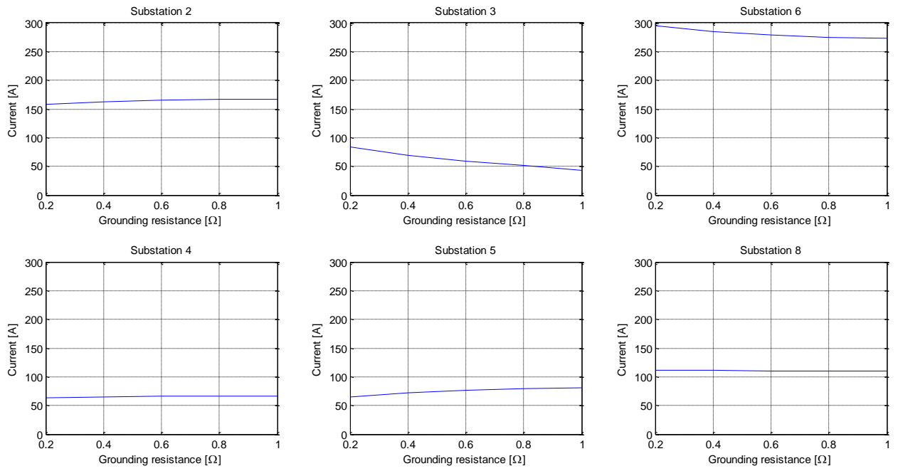
Figure 38 Induced current in different busses when modifying resistance in substation 3, full scale.
