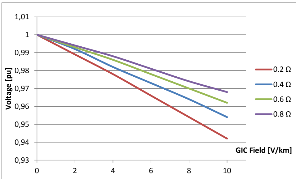
Figure 21 Voltage drop for different grounding resistance in a three legged transformer.
