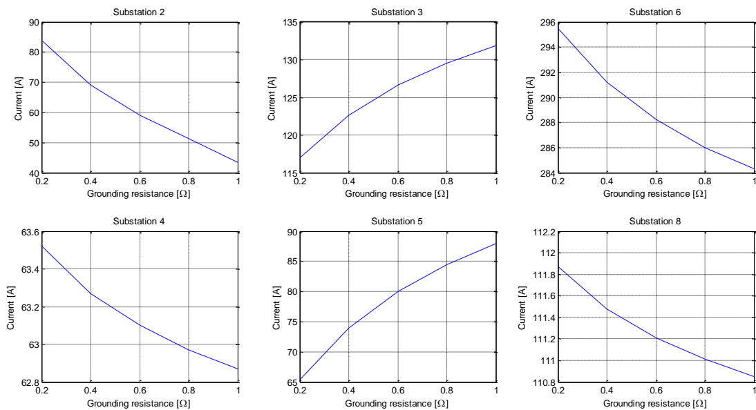
Figure 4 Induced currents in different busses when changing grounding resistance in bus 2 under a 5V/km GIC field.
