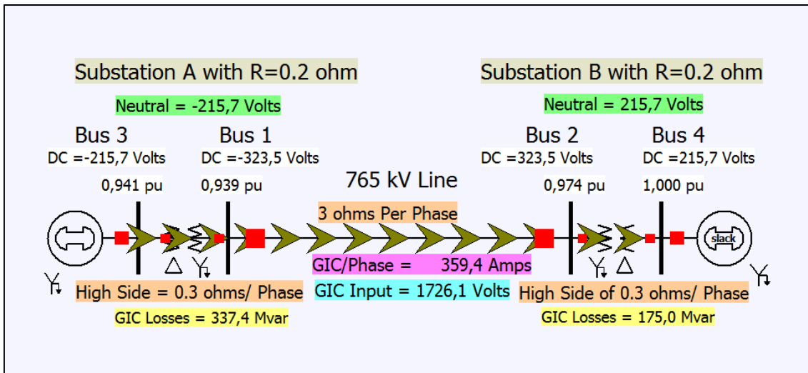
Figure 12 4 bus test system under 10 V/km GIC.
