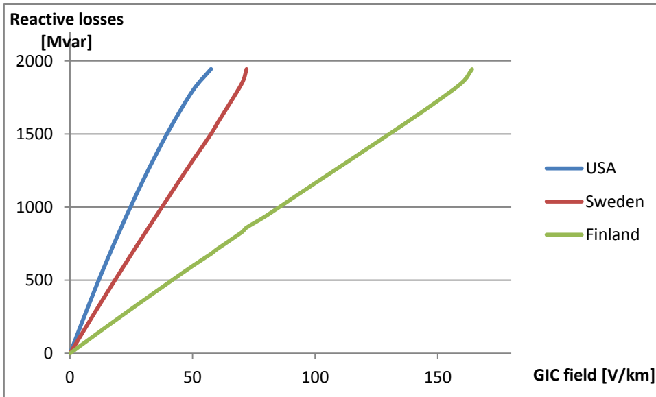
Figure 14 graph reactive losses vs GIC field between countries, transformer 2.
