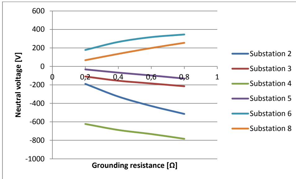
Figure 32 Neutral voltages in different buses when applying grounding resistance
