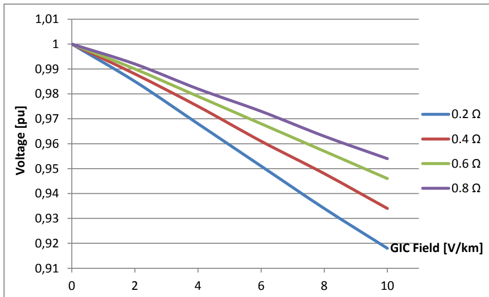
Figure 25 Voltage drop for different grounding resistance in a three legged transformer shell.
