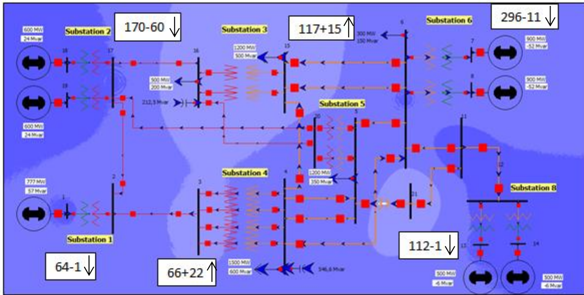
Figure 37 Induced current in different busses when modifying resistance in substation 2 [A]
