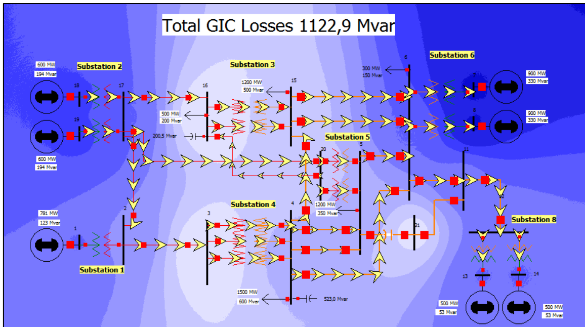
Figure 41 21 Bus system without one of the transformers in parallel.
