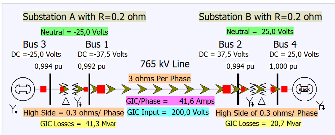
Figure 11 4-bus test system [6].
