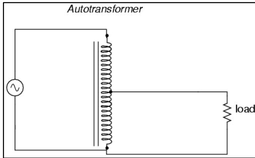
Figure 10 Autotransformer [12]
