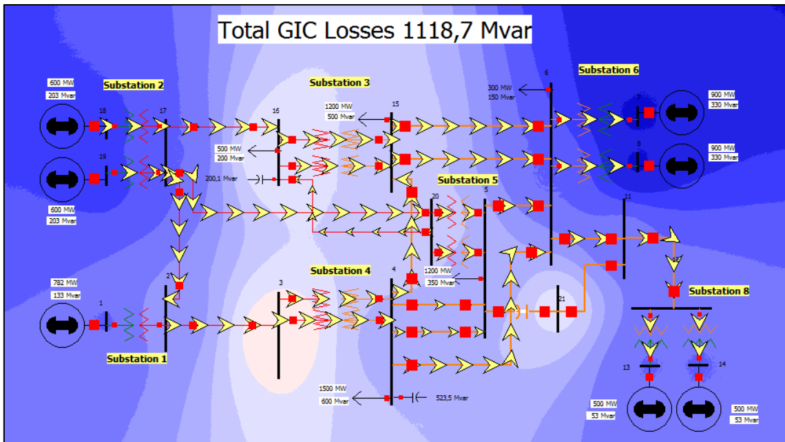
Figure 42 21 Bus system without two of the transformers in parallel.
