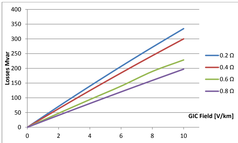
Figure 22 Reactive losses for different grounding resistance in a five legged transformer.
