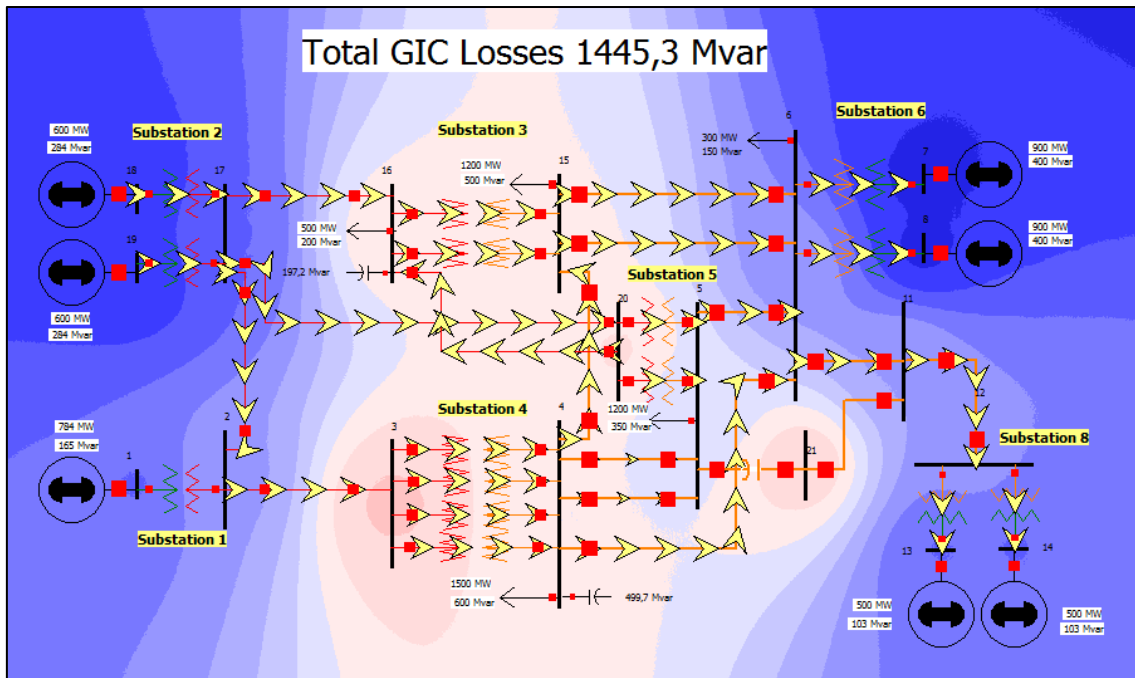
Figure 30 21 Bus system applying capacitors in three buses, substations 3, 6 and 5
