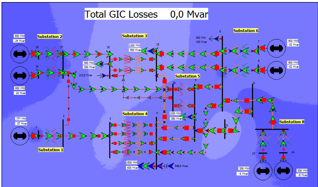
Figure 28 21 bus system under no GIC field
