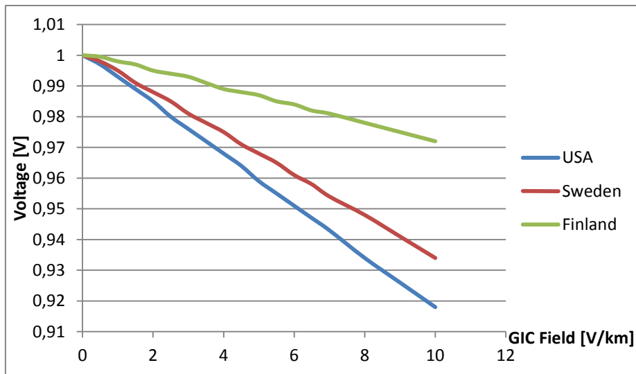
Figure 19 Comparison between countries, Voltage reduction.
