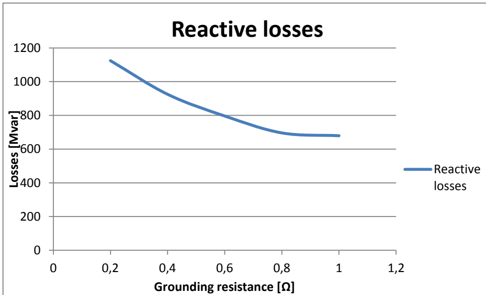
Figure 33 Reactive losses in 21 bus system when increasing grounding resistance everywhere
