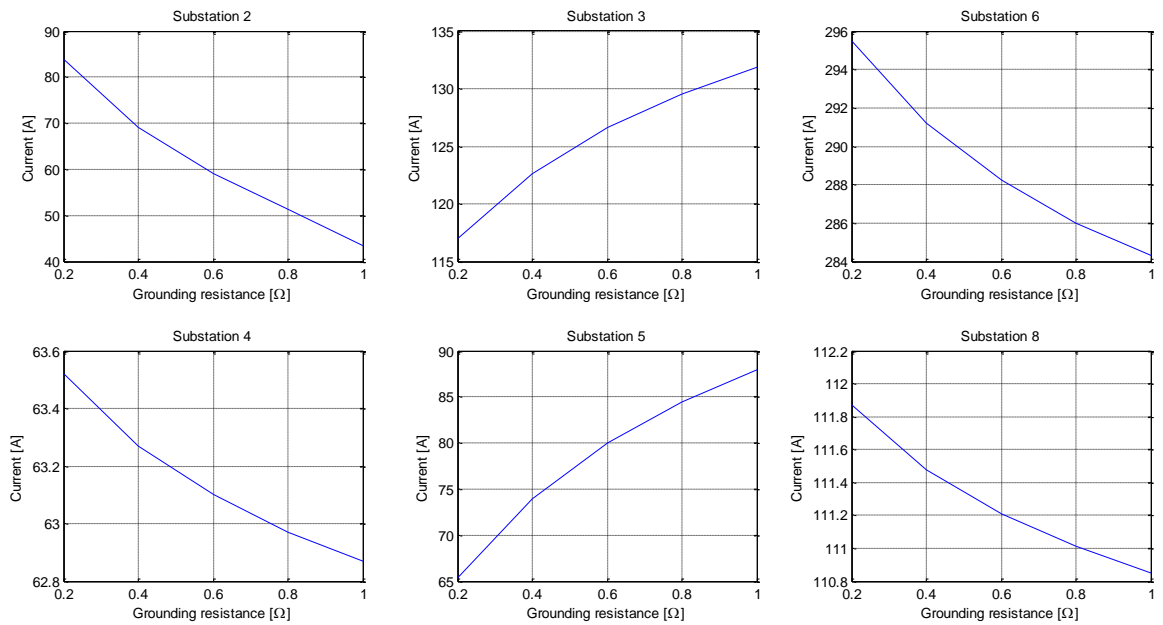
Figure 36 Induced current in different busses when modifying resistance in substation 2, magnified.
