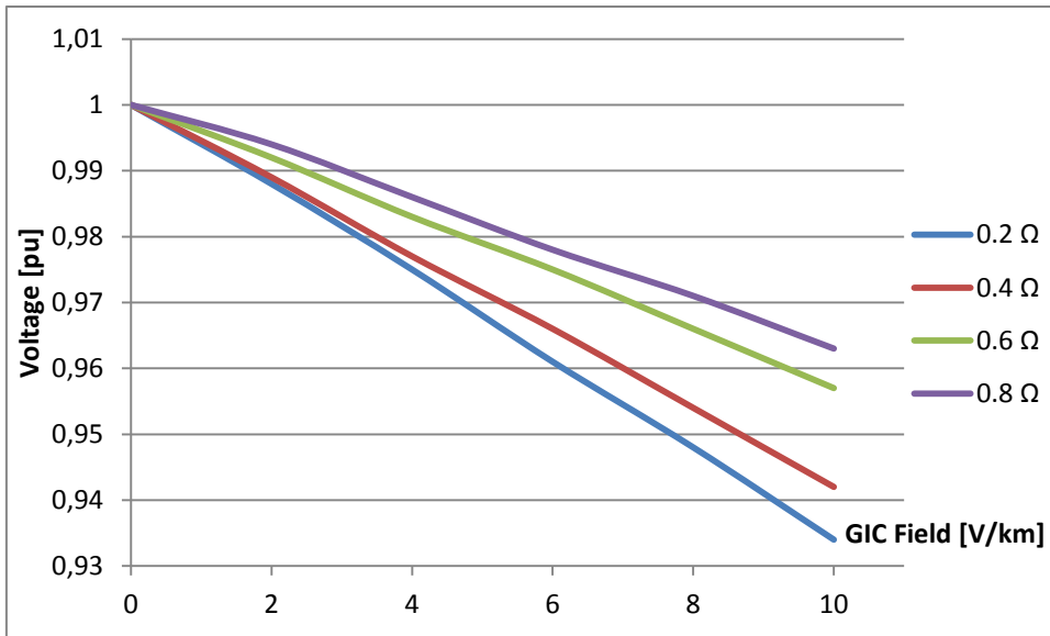
Figure 23 Voltage drop for different grounding resistance in a five-legged transformer.
