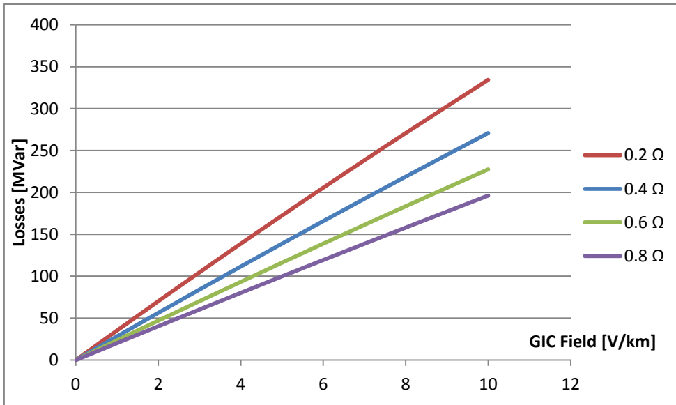
Figure 20 Reactive losses for different grounding resistance in a three legged transformer.
