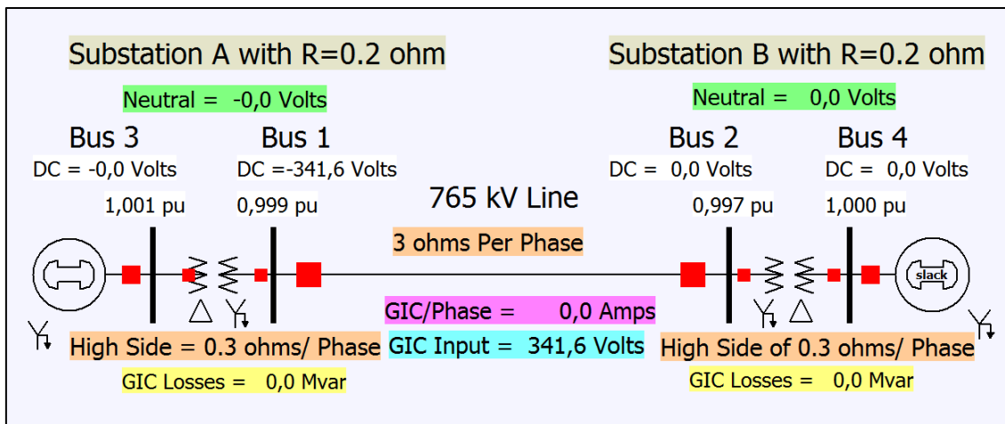
Figure 26 Delta connection working as a capacitor in the grounding of the transformer; delta connection cannot be seen due to the specifications of the software.
