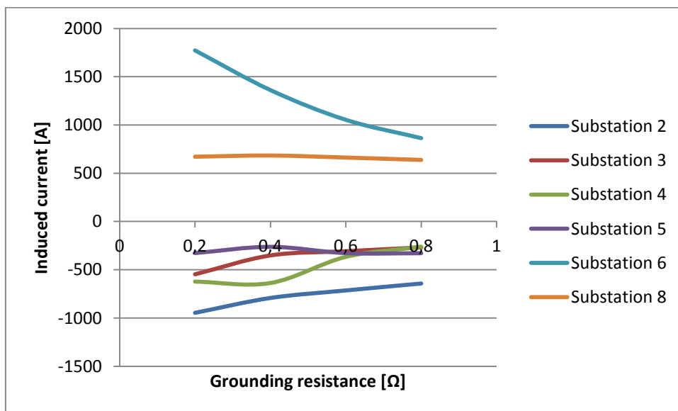
Figure 31 Induced currents in 21 bus system applying grounding resistances
