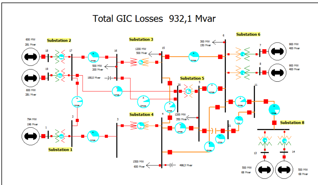
Figure 44 21 Bus system without all the possible skipped elements.
