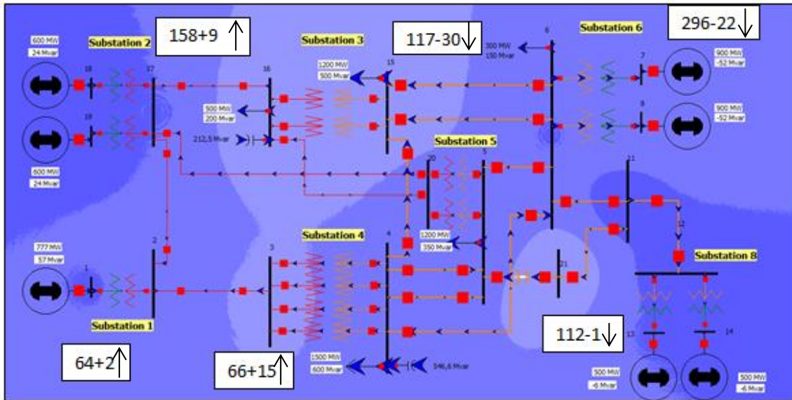
Figure 40 Induced current in different busses when modifying resistance in substation 3 [A]
