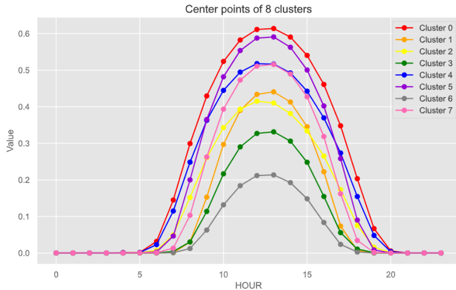
Figure 28. Centers of the 8 clusters for Solar PV generation
