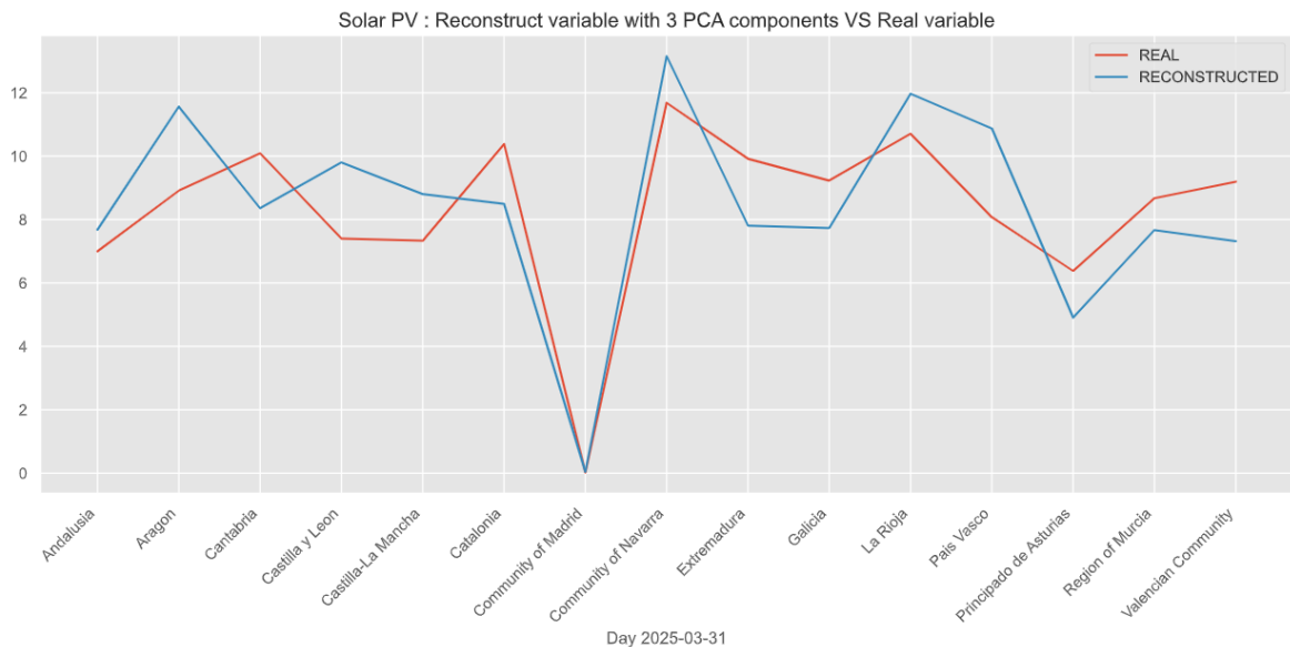
Figure 16. Reconstruct variables with the three main principal components for Solar PV daily generation
