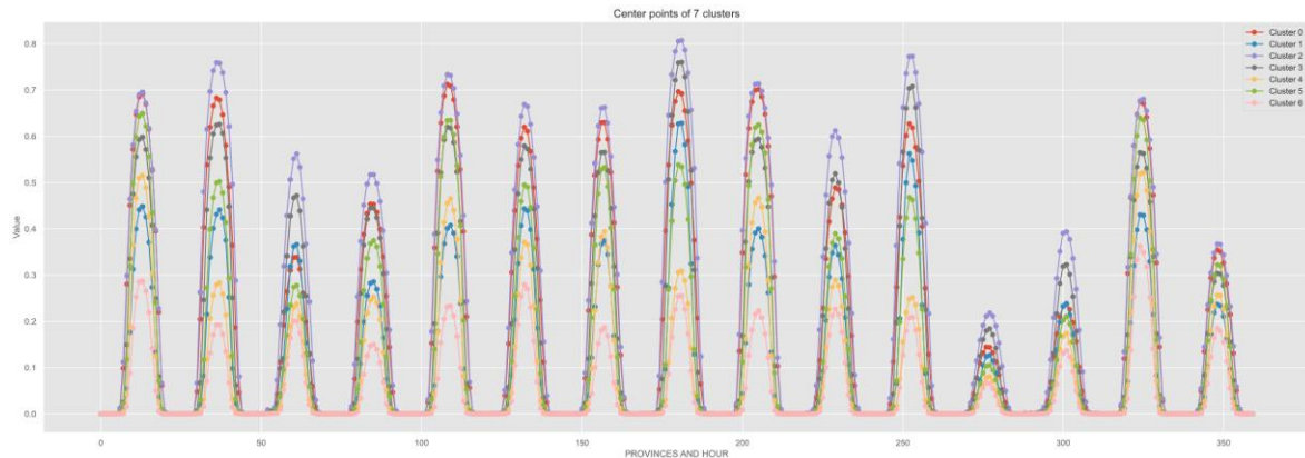
Figure 38. Center points of seven clusters for hourly Solar PV generation by provinces
