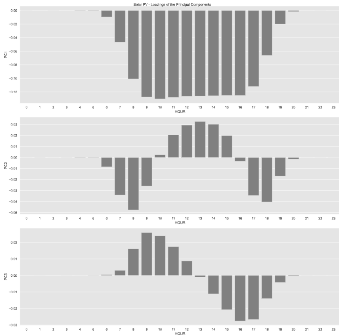
Figure 19. PCA Loadings for hourly Solar PV generation
