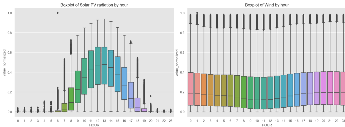
Figure 64. Box-plot of PV and Wind by hour
