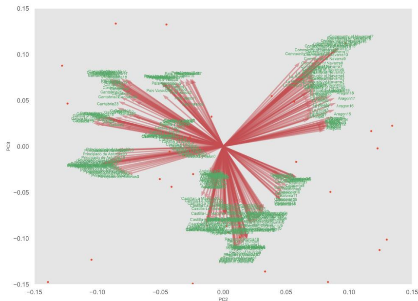
Figure 56. Biplot with PC2 and PC3 for wind generation by provinces
