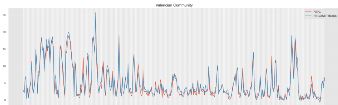
Figure 44. Reconstructed wind generation of Valencia with 5-PCs
