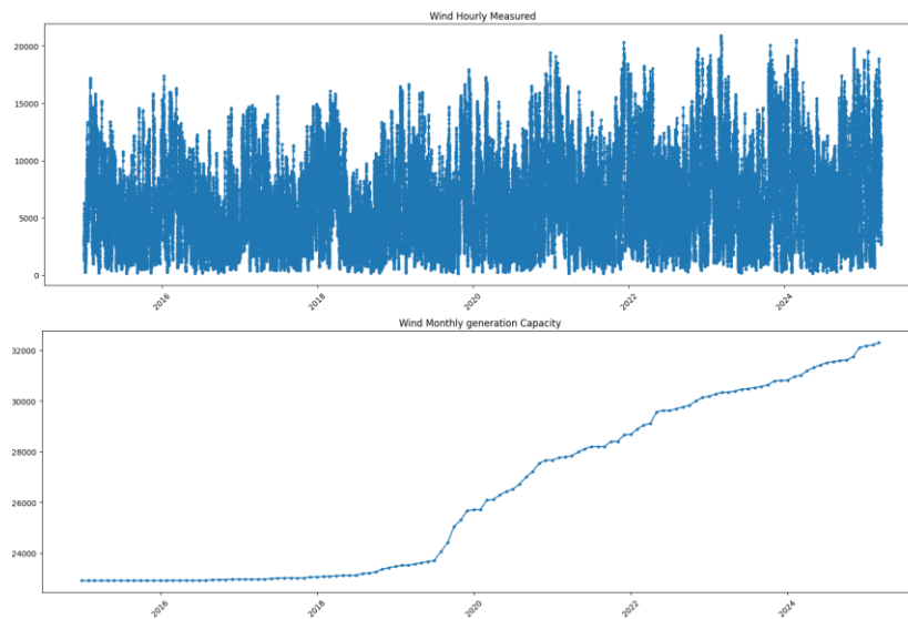
Figure 6. Wind - Measured / Capacity
