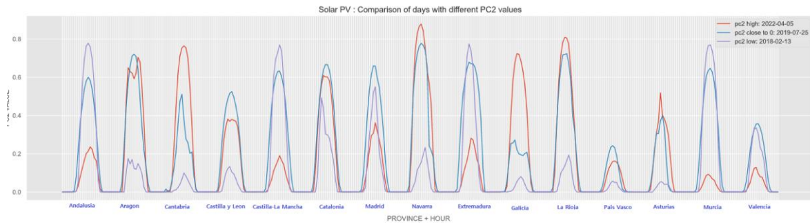
Figure 34. Three representative days according to PC2 values for Solar PV generation by provinces
