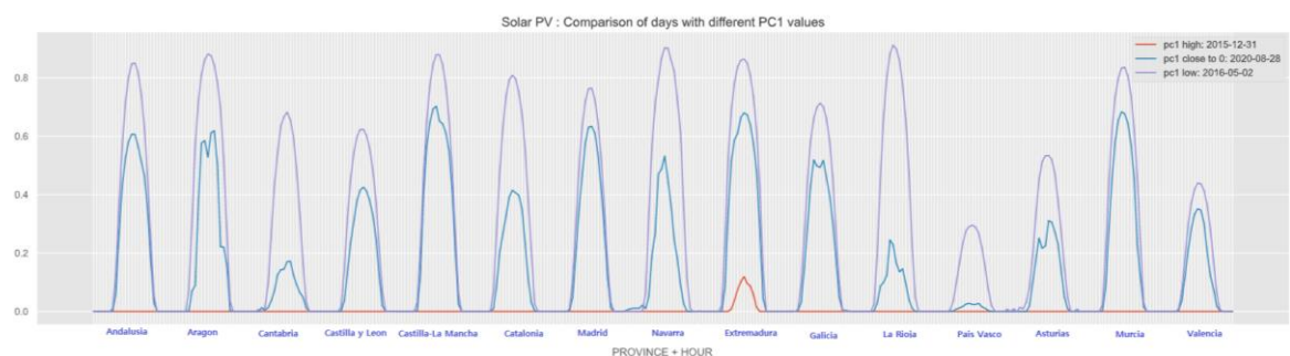
Figure 33. Three representative days according to PC1 for Solar PV generation by provinces
