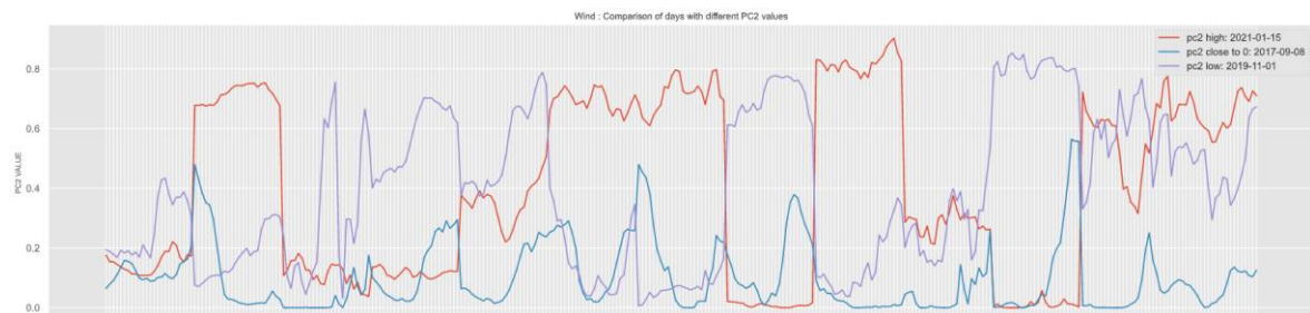
Figure 58. Three days of hourly wind generation by provinces selected according to PC2
