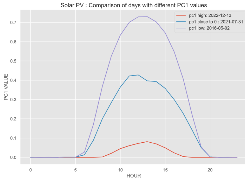
Figure 24. PC1 values with dates for Solar PV generation
