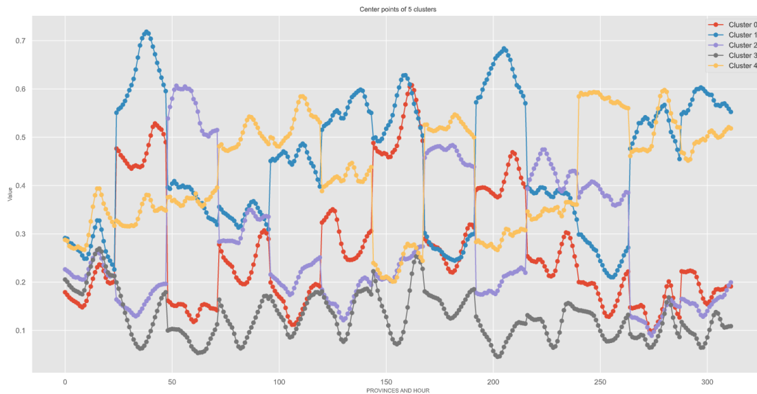
Figure 63. Main hourly patterns for wind generation by provinces
