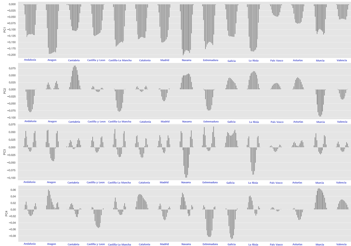
Figure 29. PCA Loadings for hourly Solar PV generation by provinces
