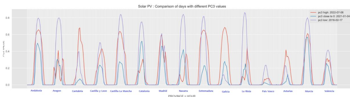
Figure 35. Three representative days according to PC3 for Solar PV generation by provinces
