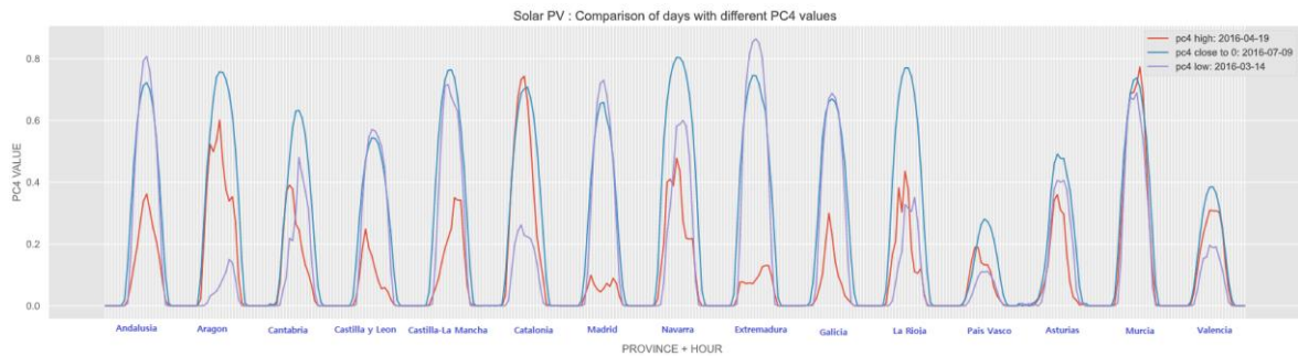
Figure 36. Three representative days according to PC4 for Solar PV generation by provinces
