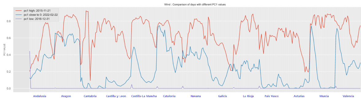
Figure 57. Three days of hourly wind generation by provinces selected according to PC1
