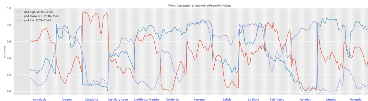
Figure 60. Three days of hourly wind generation by provinces selected according to PC4
