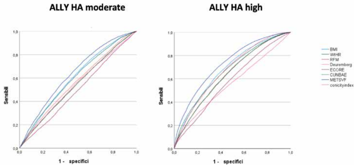
Figure 2: ROC curve.
