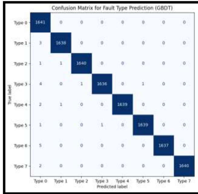
Figure 15. GBDT Scenario 2 Confusion Matrix
