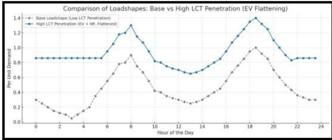
Figure 9. LCT Scenarios Load-shape
