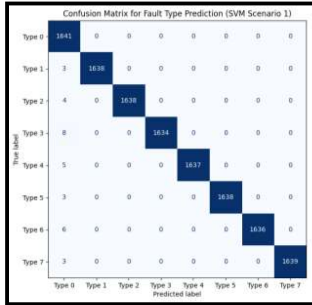
Figure 18. SVM Scenario 1 Confusion Matrix
