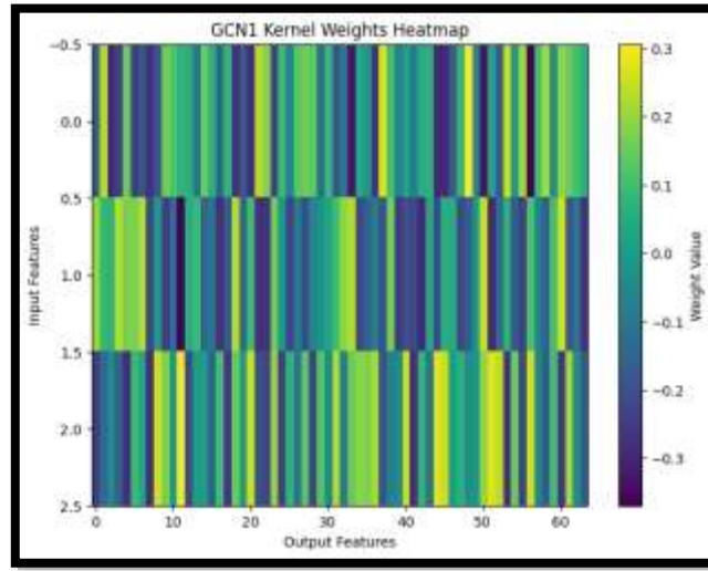
Figure 23. GNN Fault Classification kernel Weights Heat map
