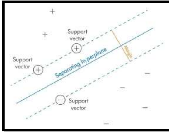
Figure 2. SVM example [13]
