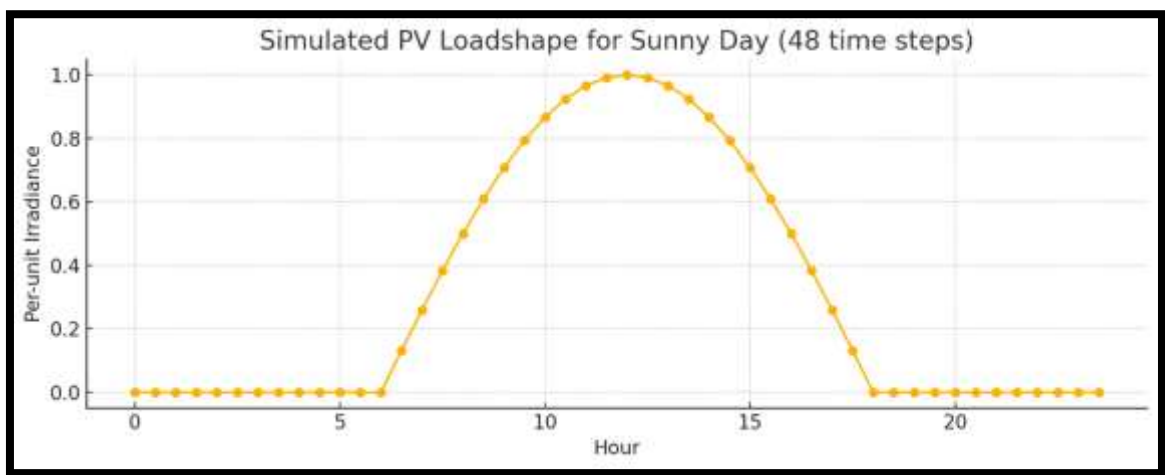
Figure 11. Solar Generation Curve
