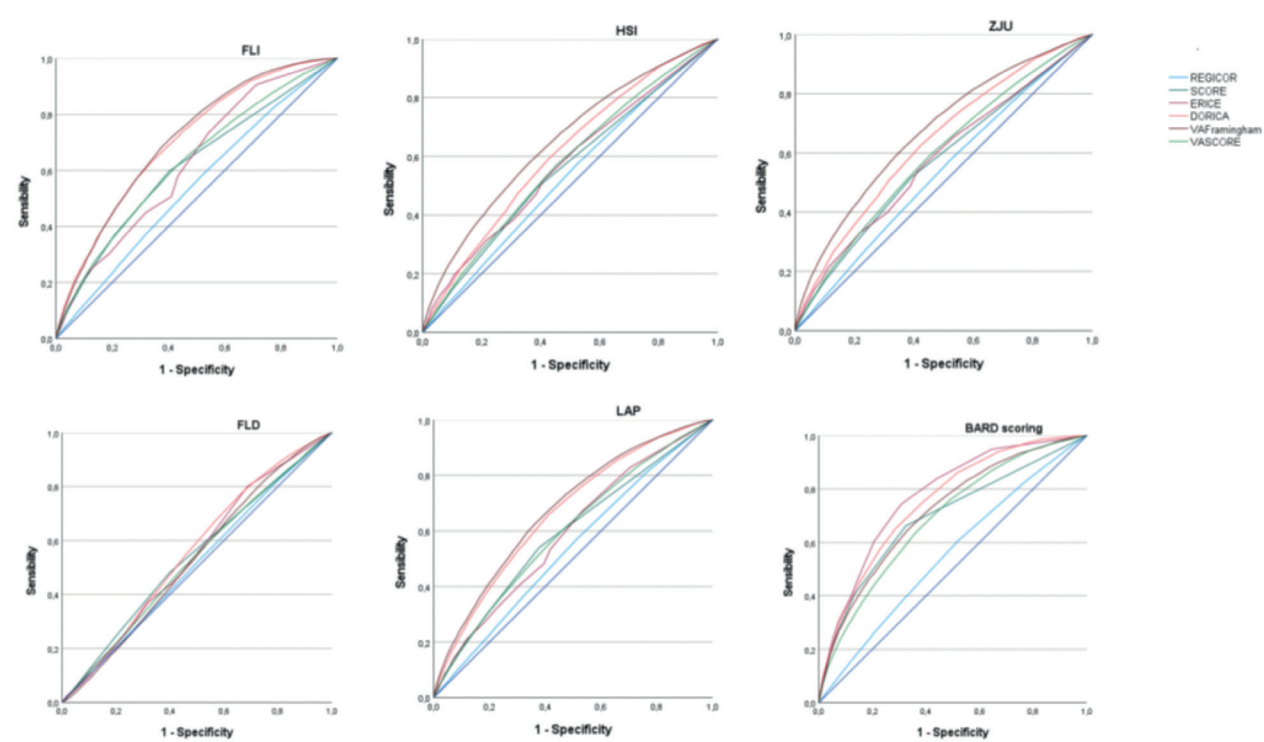
Figure 2: ROC curve.
