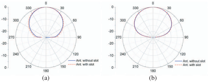
Figure 3. (a) Radiation pattern of the designed patch antennas for electric plane XZ and (b) for magnetic plane YZ . The normalized gains are 7.7 dBi and 8 dBi for the patch antenna without slot and the same antenna with slot, respectively.
