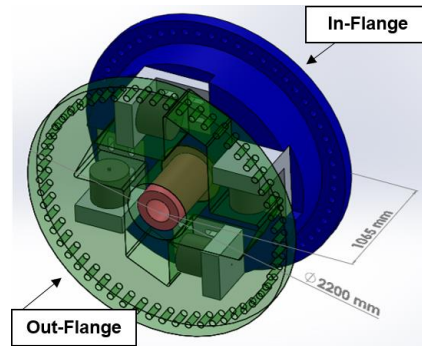
Figure 3. Proposed force lever system.
