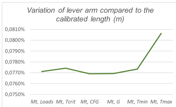
Figure 6. Variation of the lever length
