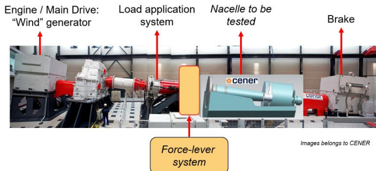
Figure 2. Nacelle Test Bench and position of LAS and FLS.
