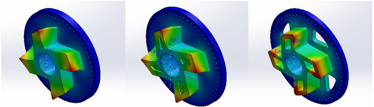
Figure 4. Lever arm improvements (from original concept to the final design).
