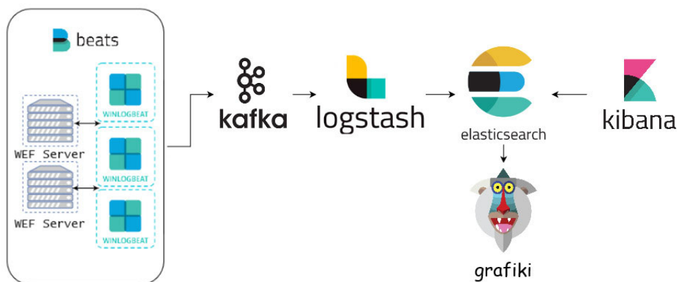
Figure 2. Event Based Detection System (EBDS) Diagram.
