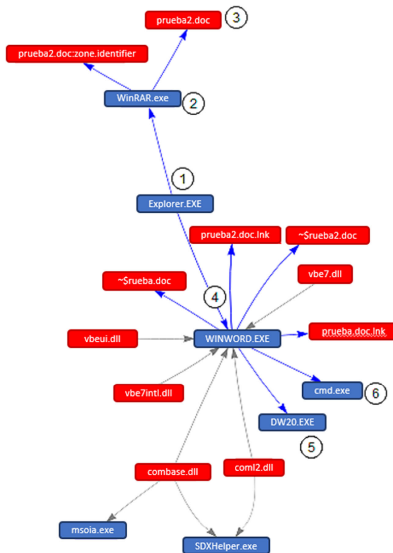
Figure 3. Result of malicious macro execution in a Microsoft Word document.
