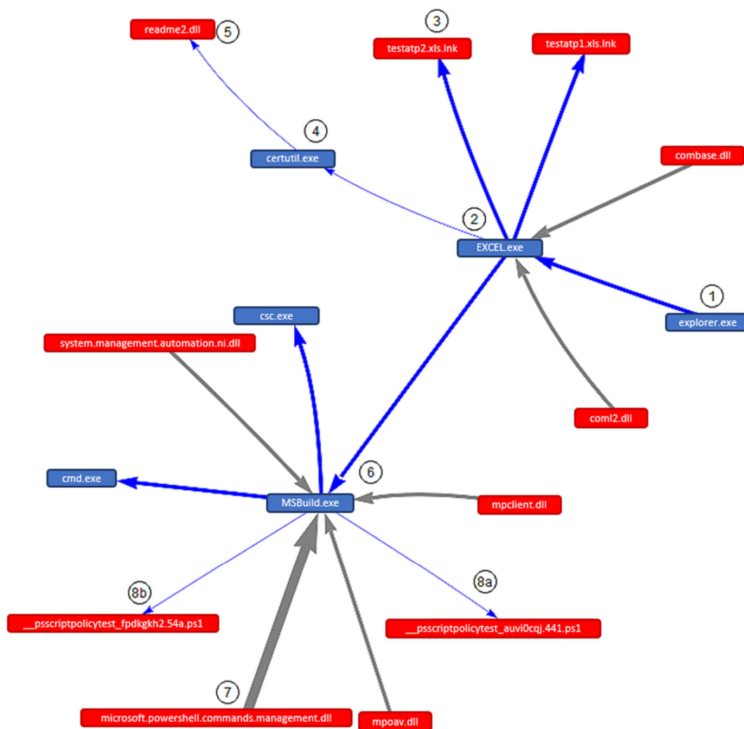
Figure 5. Result of Excel document execution with CertUtil.exe and MSBuild.exe.
