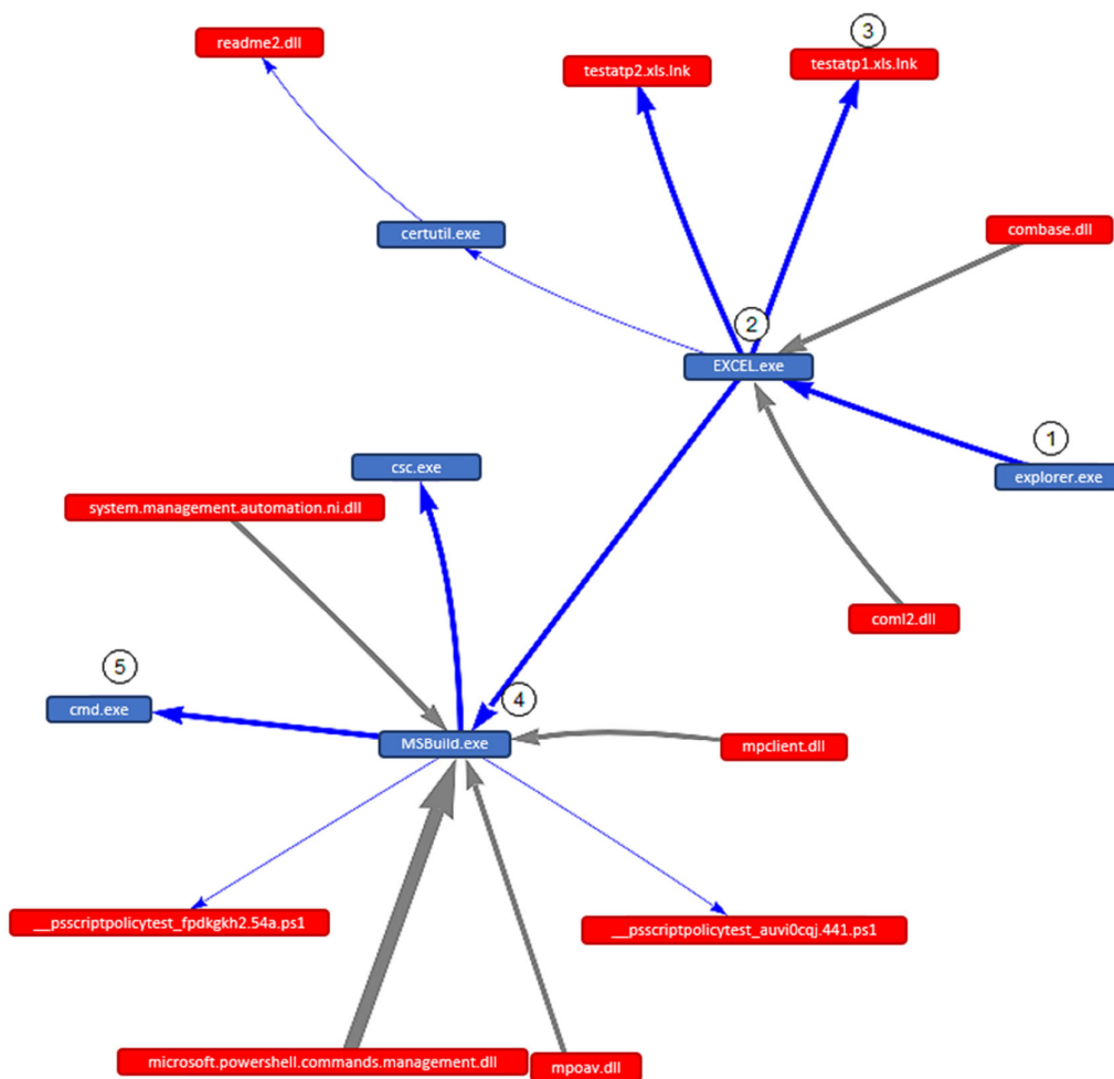
Figure 4. Result of the execution of an Excel document with MSBuild.exe.
